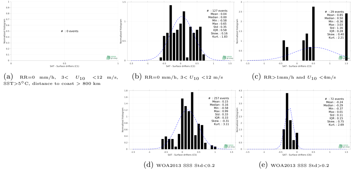
Figure 12: Normalized histogram of \Delta SSS (Aquarius SSS L3 OR v5 - Monthly (NASA-GSFC) - Surface drifters) for 5 different subdatasets corresponding to: RR=0 mm/h, 3 < U_{10} < 12 m/s, SST > 5°C, distance to coast > 800 km (a), RR=0 mm/h, 3 < U_{10} < 12 m/s (b), RR > 1mm/h and U_{10} < 4 m/s (c), WOA2013 SSS Std < 0.2 (d), WOA2013 SSS Std > 0.2 (e).
