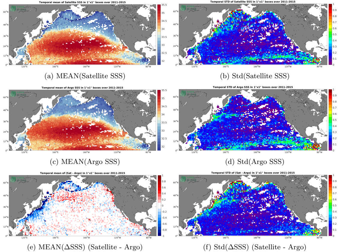
Figure 6: Temporal mean (left) and Std (right) of SSS from Aquarius SSS L3 OR v5 - Monthly (NASA-GSFC) (top), Argo (middle), and of \Delta\text{SSS} (Satellite - Argo). Only match-up pairs are used to generate these maps.
