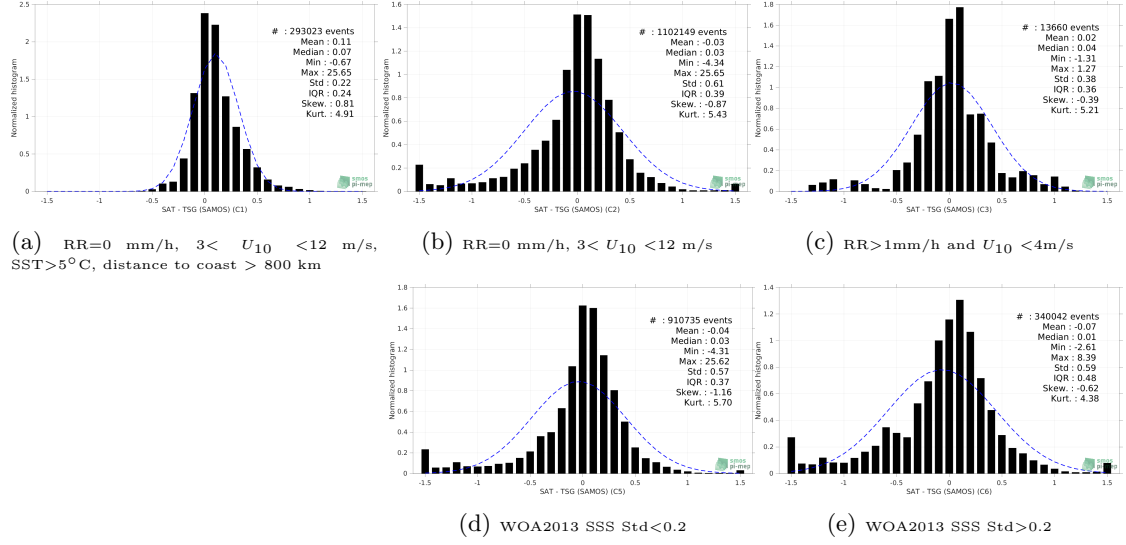
Figure 13: Normalized histogram of \Delta\text{SSS} (Aquarius SSS L3 OR v5 - Monthly - Rain mask (NASA-GSFC) - TSG (SAMOS)) for 5 different subdatasets corresponding to: RR=0 mm/h, 3 < U_{10} < 12 m/s, SST>5°C, distance to coast > 800 km (a), RR=0 mm/h, 3 < U_{10} < 12 m/s (b), RR>1mm/h and U_{10} < 4 m/s (c), WOA2013 SSS Std<0.2 (d), WOA2013 SSS Std>0.2 (e).
