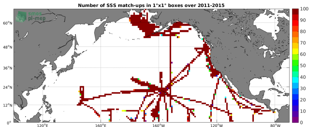
Figure 4: Number of SSS match-ups between TSG-SAMOS SSS and the Aquarius-L3-OR-V5-MONTHLY-RAIN-MASK-1DEG SSS product for the North Pacific Ocean Pi-MEP region over 1°x1° boxes and for the full satellite product period.
