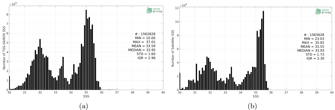
Figure 2: Histograms of SSS from TSG-SAMOS (a) and Aquarius-L3-OR-V5-MONTHLY-RAIN-MASK-1DEG (b) considering all match-up pairs per bins of 0.1 over the North Pacific Ocean Pi-MEP region and for the full satellite product period.
