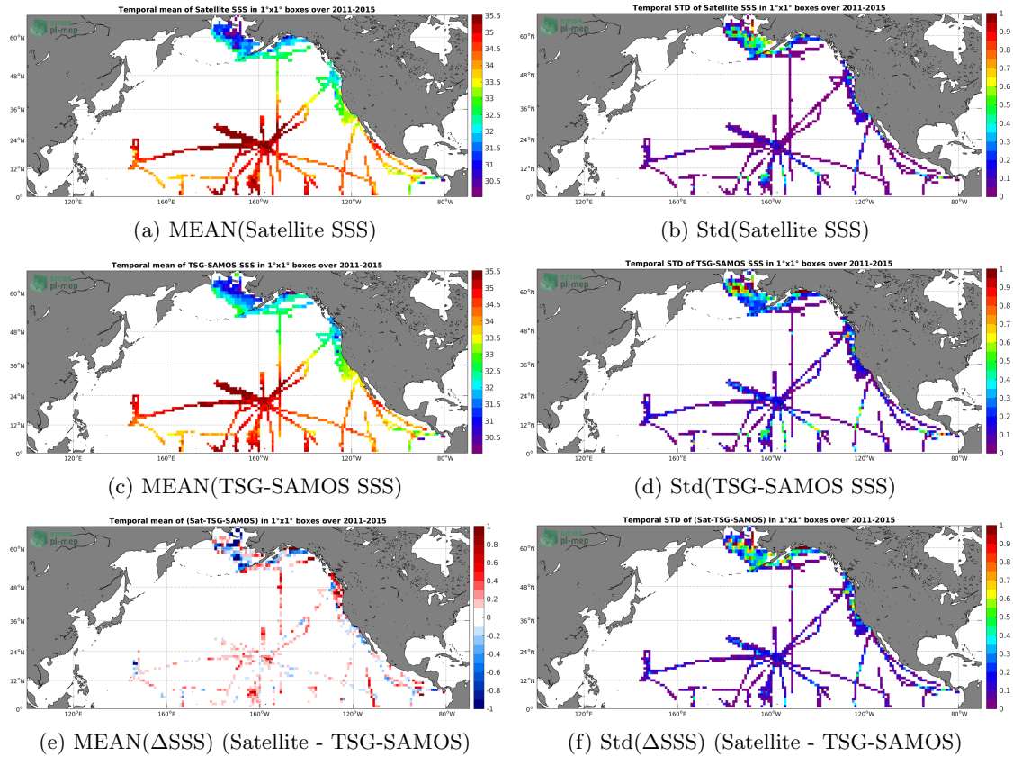
Figure 6: Temporal mean (left) and Std (right) of SSS from Aquarius-L3-OR-V5-MONTHLY-RAIN-MASK-1DEG (top), TSG-SAMOS (middle), and of \Delta SSS (Satellite - TSG-SAMOS). Only match-up pairs are used to generate these maps.
