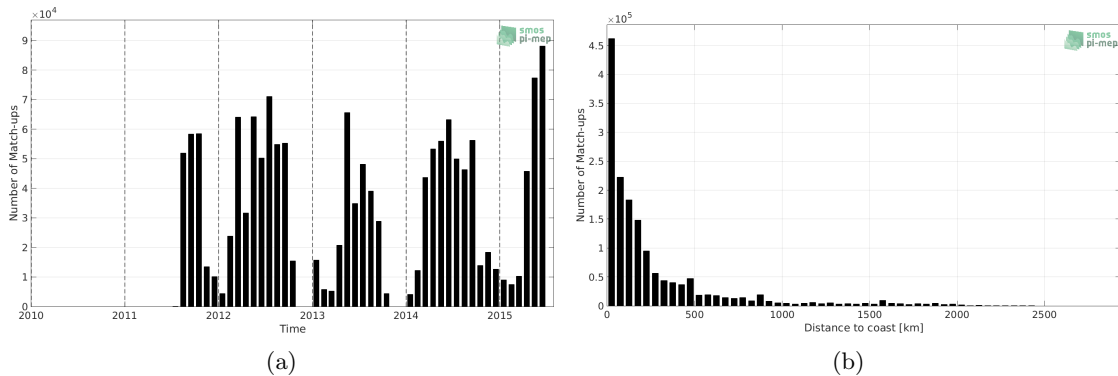
Figure 1: Number of match-ups between TSG-SAMOS and Aquarius-L3-OR-V5-MONTHLY-RAIN-MASK-1DEG SSS as a function of time (a) and as function of the distance to coast (b) over the North Pacific Ocean Pi-MEP region and for the full satellite product period.
