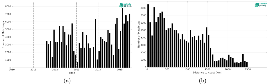
Figure 2: Number of match-ups between TSG (LEGOS-DM) and Aquarius SSS L3 OR v5 - Monthly - Rain mask (NASA-GSFC) SSS as a function of time (a) and as function of the distance to coast (b) over the North Pacific Ocean Pi-MEP region and for the full satellite product period.
