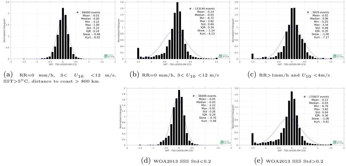
Figure 13: Normalized histogram of \Delta\text{SSS} (Aquarius-L3-OR-V5-MONTHLY-RAIN-MASK-1DEG - TSG-LEGOS-DM) for 5 different subdatasets corresponding to: RR=0 mm/h, 3 < U_{10} < 12 m/s, SST > 5^\circ\text{C} , distance to coast > 800 km (a), RR=0 mm/h, 3 < U_{10} < 12 m/s (b), RR > 1 mm/h and U_{10} < 4 m/s (c), WOA2013 SSS Std < 0.2 (d), WOA2013 SSS Std > 0.2 (e).
