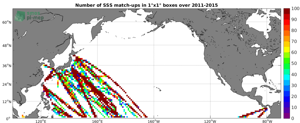
Figure 4: Number of SSS match-ups between TSG-LEGOS-DM SSS and the Aquarius-L3-OR-V5-MONTHLY-RAIN-MASK-1DEG SSS product for the North Pacific Ocean Pi-MEP region over 1^\circ \times 1^\circ boxes and for the full satellite product period.
