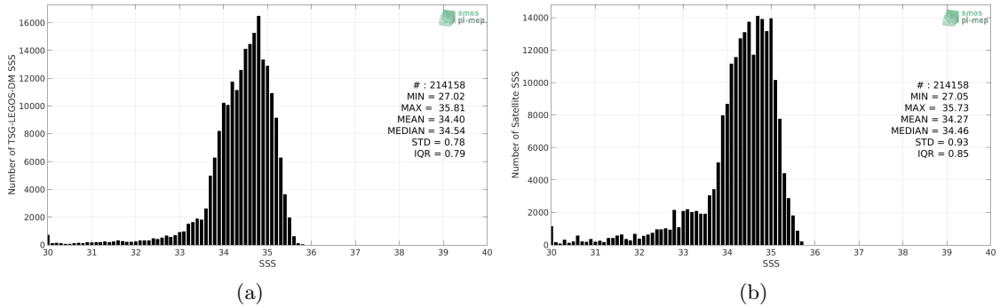
Figure 2: Histograms of SSS from TSG-LEGOS-DM (a) and Aquarius-L3-OR-V5-MONTHLY-RAIN-MASK-1DEG (b) considering all match-up pairs per bins of 0.1 over the North Pacific Ocean Pi-MEP region and for the full satellite product period.
