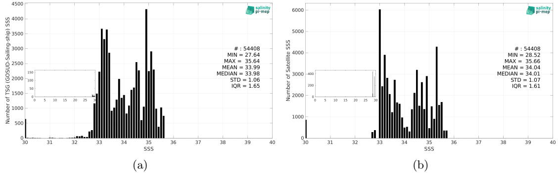
Figure 3: Histograms of SSS from TSG (GOSUD-Sailing-ship) (a) and Aquarius SSS L3 OR v5 - Monthly - Rain mask (NASA-GSFC) (b) considering all match-up pairs per bins of 0.1 over the North Pacific Ocean Pi-MEP region and for the full satellite product period.
