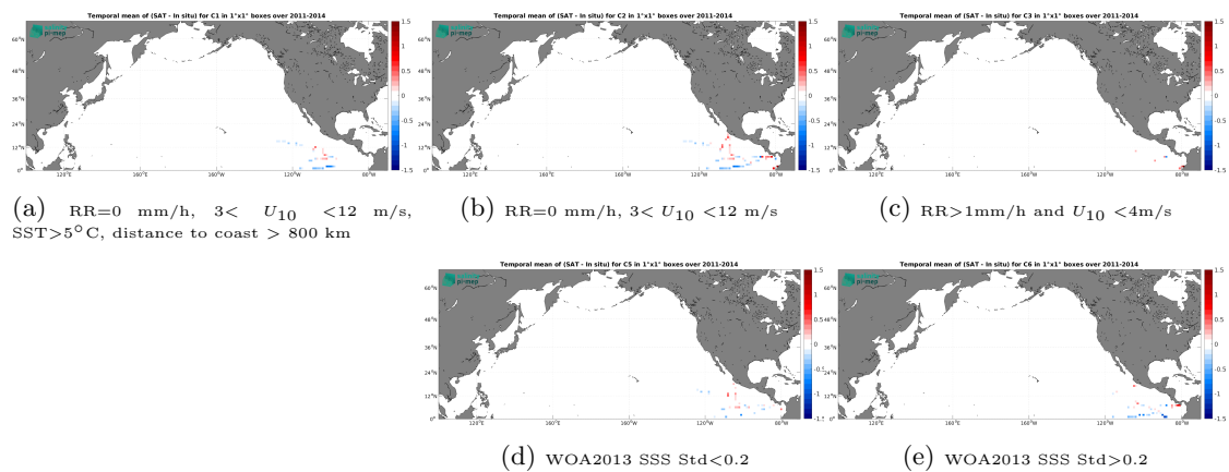
Figure 14: Temporal mean gridded over spatial boxes of size 1^\circ \times 1^\circ of \Delta\text{SSS} (Aquarius SSS L3 OR v5 - Monthly - Rain mask (NASA-GSFC) - TSG (GOSUD-Research-vessel)) for 5 different subdatasets corresponding to: RR=0 mm/h, 3 < U_{10} < 12 m/s, SST > 5°C, distance to coast > 800 km (a), RR=0 mm/h, 3 < U_{10} < 12 m/s (b), RR > 1mm/h and U_{10} < 4 m/s (c), WOA2013 SSS Std < 0.2 (d), WOA2013 SSS Std > 0.2 (e).
