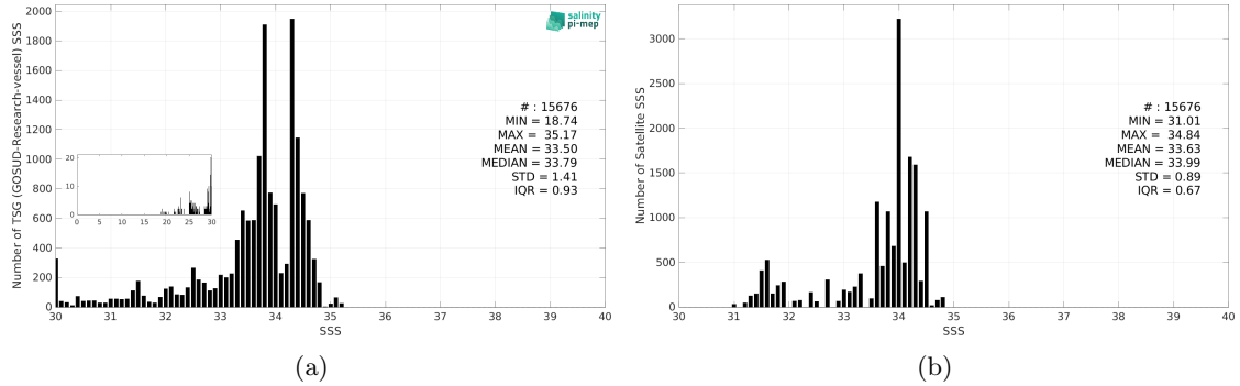
Figure 3: Histograms of SSS from TSG (GOSUD-Research-vessel) (a) and Aquarius SSS L3 OR v5 - Monthly - Rain mask (NASA-GSFC) (b) considering all match-up pairs per bins of 0.1 over the North Pacific Ocean Pi-MEP region and for the full satellite product period.
