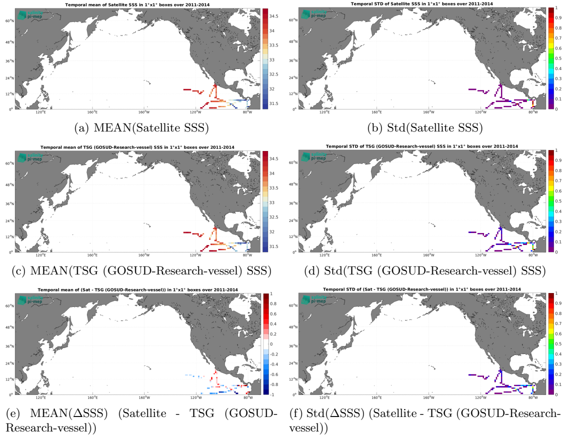
Figure 7: Temporal mean (left) and Std (right) of SSS from Aquarius SSS L3 OR v5 - Monthly - Rain mask (NASA-GSFC) (top), TSG (GOSUD-Research-vessel) (middle), and of \Delta\text{SSS} (Satellite - TSG (GOSUD-Research-vessel)). Only match-up pairs are used to generate these maps.
