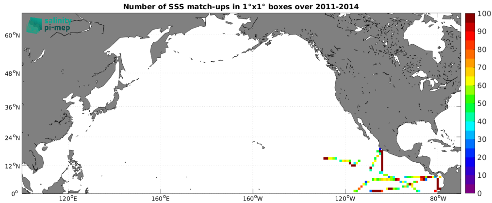
Figure 5: Number of SSS match-ups between TSG (GOSUD-Research-vessel) SSS and the Aquarius SSS L3 OR v5 - Monthly - Rain mask (NASA-GSFC) SSS product for the North Pacific Ocean Pi-MEP region over 1^\circ \times 1^\circ boxes and for the full satellite product period.
