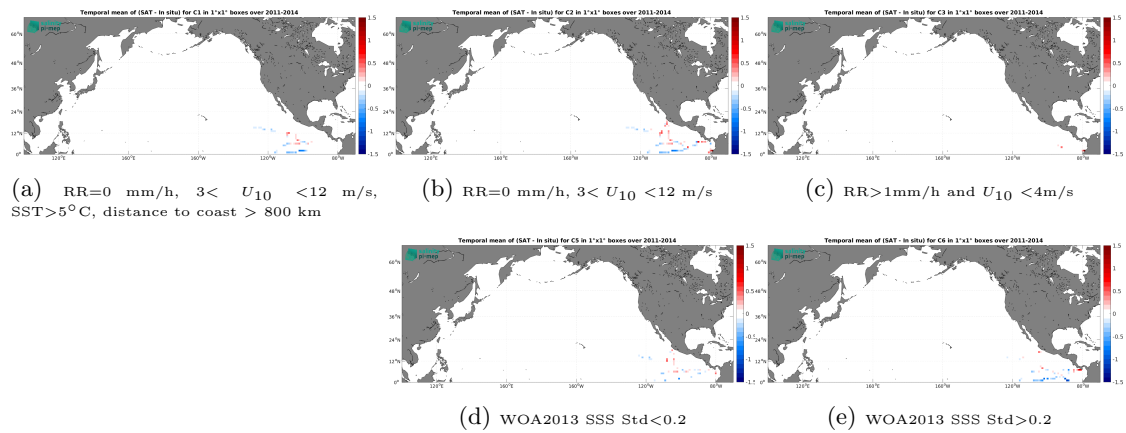
Figure 12: Temporal mean gridded over spatial boxes of size 1^\circ \times 1^\circ of \Delta\text{SSS} (Aquarius SSS L3 OR v5 - Monthly - Rain mask (NASA-GSFC) - TSG (GOSUD-Research-vessel)) for 5 different subdatasets corresponding to: RR=0 mm/h, 3 < U_{10} < 12 m/s, SST > 5°C, distance to coast > 800 km (a), RR=0 mm/h, 3 < U_{10} < 12 m/s (b), RR > 1 mm/h and U_{10} < 4 m/s (c), WOA2013 SSS Std < 0.2 (d), WOA2013 SSS Std > 0.2 (e).
