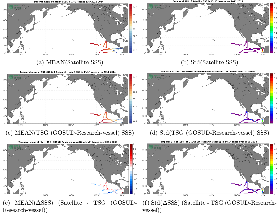
Figure 6: Temporal mean (left) and Std (right) of SSS from Aquarius SSS L3 OR v5 - Monthly - Rain mask (NASA-GSFC) (top), TSG (GOSUD-Research-vessel) (middle), and of \Delta SSS (Satellite - TSG (GOSUD-Research-vessel)). Only match-up pairs are used to generate these maps.
