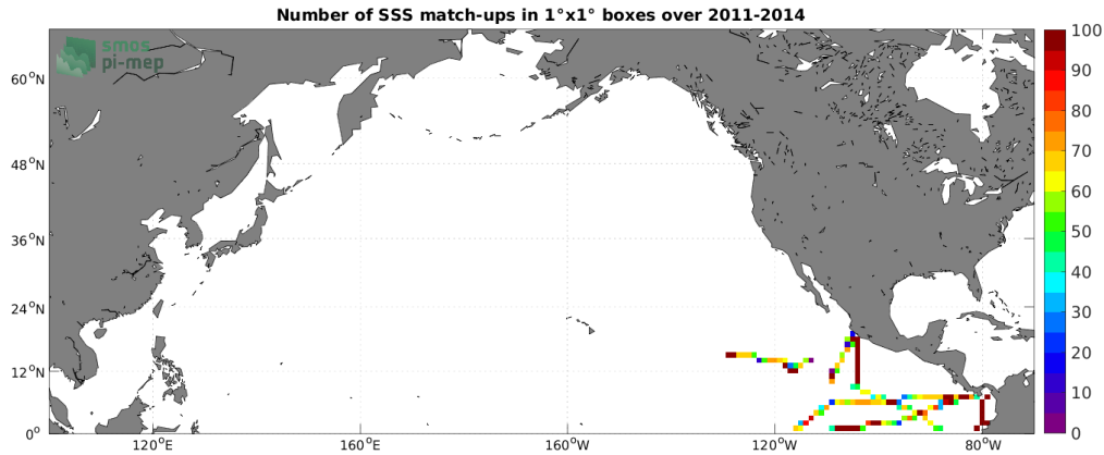
Figure 4: Number of SSS match-ups between TSG (GOSUD-Research-vessel) SSS and the Aquarius SSS L3 OR v5 - Monthly - Rain mask (NASA-GSFC) SSS product for the North Pacific Ocean Pi-MEP region over 1^\circ \times 1^\circ boxes and for the full satellite product period.
