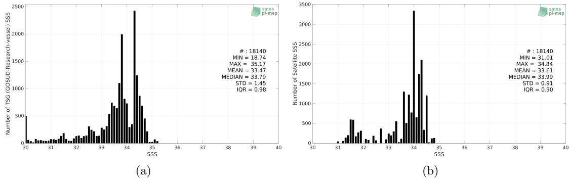
Figure 2: Histograms of SSS from TSG (GOSUD-Research-vessel) (a) and Aquarius SSS L3 OR v5 - Monthly - Rain mask (NASA-GSFC) (b) considering all match-up pairs per bins of 0.1 over the North Pacific Ocean Pi-MEP region and for the full satellite product period.
