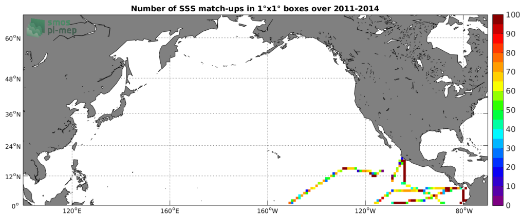
Figure 4: Number of SSS match-ups between TSG-GOSUD-Research-vessel SSS and the Aquarius-L3-OR-V5-MONTHLY-RAIN-MASK-1DEG SSS product for the North Pacific Ocean Pi-MEP region over 1^\circ \times 1^\circ boxes and for the full satellite product period.
