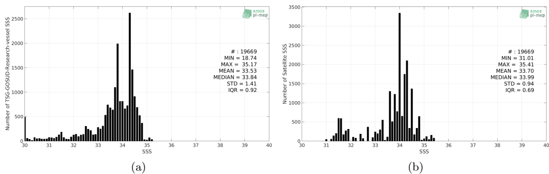
Figure 2: Histograms of SSS from TSG-GOSUD-Research-vessel (a) and Aquarius-L3-OR-V5-MONTHLY-RAIN-MASK-1DEG (b) considering all match-up pairs per bins of 0.1 over the North Pacific Ocean Pi-MEP region and for the full satellite product period.
