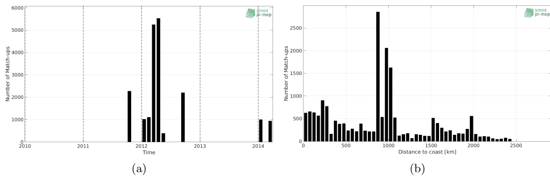
Figure 1: Number of match-ups between TSG-GOSUD-Research-vessel and Aquarius-L3-OR-V5-MONTHLY-RAIN-MASK-1DEG SSS as a function of time (a) and as function of the distance to coast (b) over the North Pacific Ocean Pi-MEP region and for the full satellite product period.
