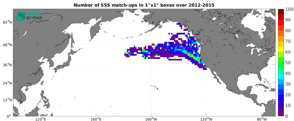
Figure 5: Number of SSS match-ups between Marine mammals SSS and the Aquarius SSS L3 OR v5 - Monthly - Rain mask (NASA-GSFC) SSS product for the North Pacific Ocean Pi-MEP region over 1°x1° boxes and for the full satellite product period.
