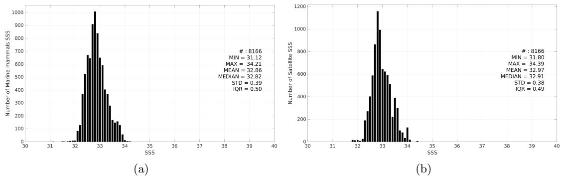
Figure 3: Histograms of SSS from Marine mammals (a) and Aquarius SSS L3 OR v5 - Monthly - Rain mask (NASA-GSFC) (b) considering all match-up pairs per bins of 0.1 over the North Pacific Ocean Pi-MEP region and for the full satellite product period.
