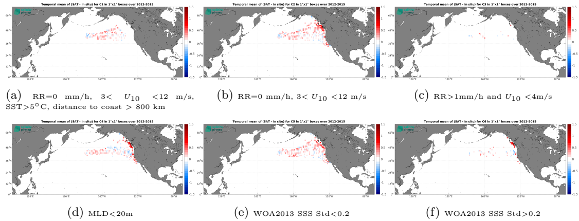
Figure 14: Temporal mean gridded over spatial boxes of size 1^\circ \times 1^\circ of \Delta SSS (Aquarius SSS L3 OR v5 - Monthly - Rain mask (NASA-GSFC) - Marine mammals) for 6 different subdatasets corresponding to:RR=0 mm/h, 3 < U_{10} < 12 m/s, SST >5^\circ C, distance to coast > 800 km (a), RR=0 mm/h, 3 < U_{10} < 12 m/s (b), RR >1 mm/h and U_{10} < 4 m/s (c),MLD <20 m (d),WOA2013 SSS Std <0.2 (e),WOA2013 SSS Std >0.2 (f).
