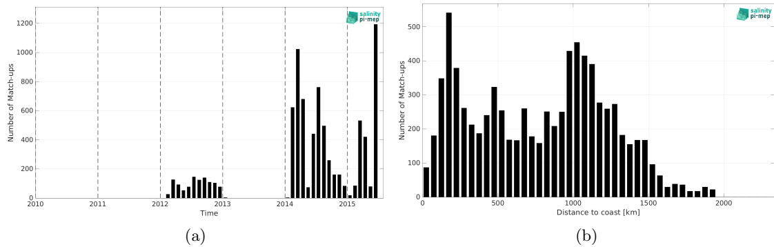
Figure 2: Number of match-ups between Marine mammals and Aquarius SSS L3 OR v5 - Monthly - Rain mask (NASA-GSFC) SSS as a function of time (a) and as function of the distance to coast (b) over the North Pacific Ocean Pi-MEP region and for the full satellite product period.
