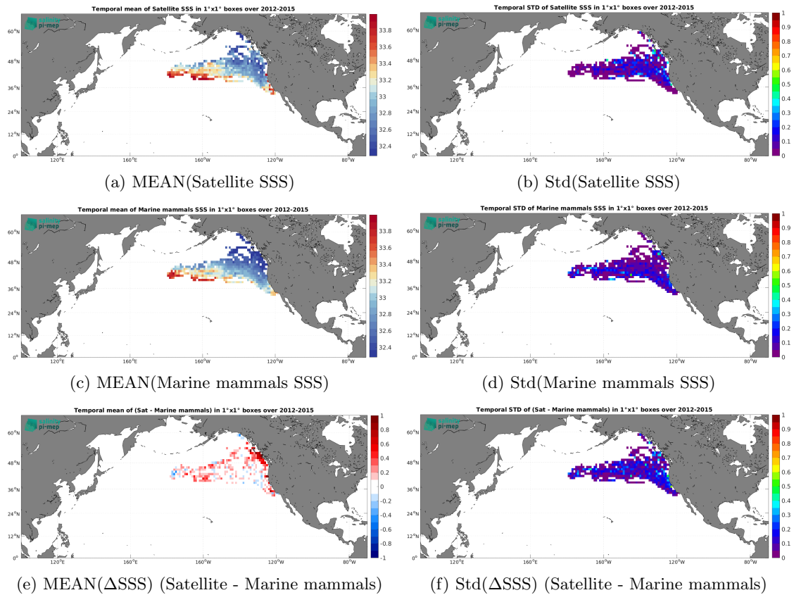
Figure 7: Temporal mean (left) and Std (right) of SSS from Aquarius SSS L3 OR v5 - Monthly - Rain mask (NASA-GSFC) (top), Marine mammals (middle), and of \Delta SSS (Satellite - Marine mammals). Only match-up pairs are used to generate these maps.
