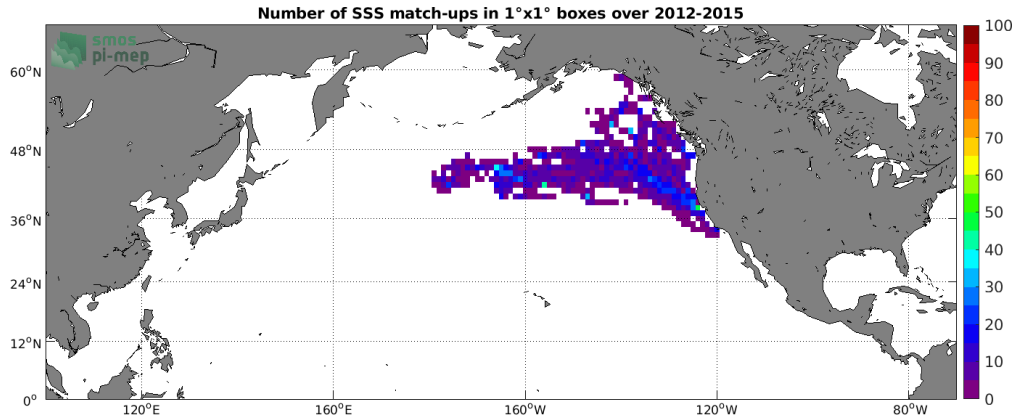
Figure 4: Number of SSS match-ups between Sea mammals SSS and the Aquarius SSS L3 OR v5 - Monthly - Rain mask (NASA-GSFC) SSS product for the North Pacific Ocean Pi-MEP region over 1^\circ \times 1^\circ boxes and for the full satellite product period.
