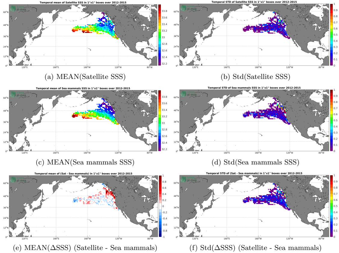
Figure 6: Temporal mean (left) and Std (right) of SSS from Aquarius SSS L3 OR v5 - Monthly - Rain mask (NASA-GSFC) (top), Sea mammals (middle), and of \Delta\text{SSS} (Satellite - Sea mammals). Only match-up pairs are used to generate these maps.
