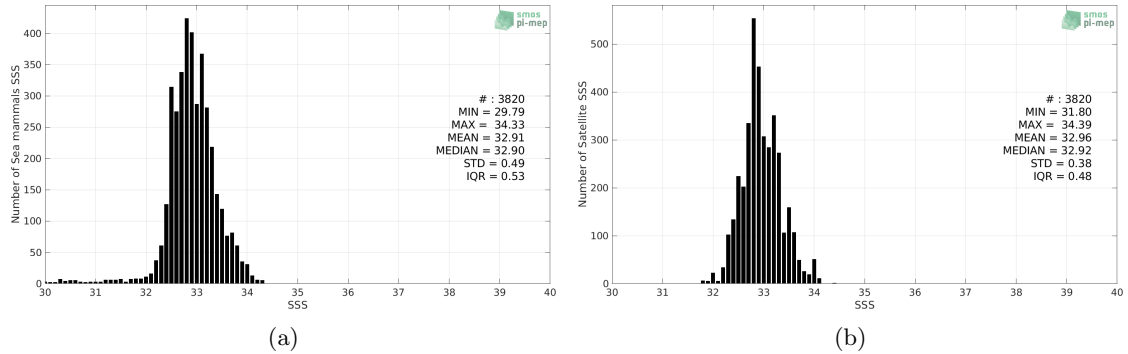
Figure 2: Histograms of SSS from Sea mammals (a) and Aquarius SSS L3 OR v5 - Monthly - Rain mask (NASA-GSFC) (b) considering all match-up pairs per bins of 0.1 over the North Pacific Ocean Pi-MEP region and for the full satellite product period.
