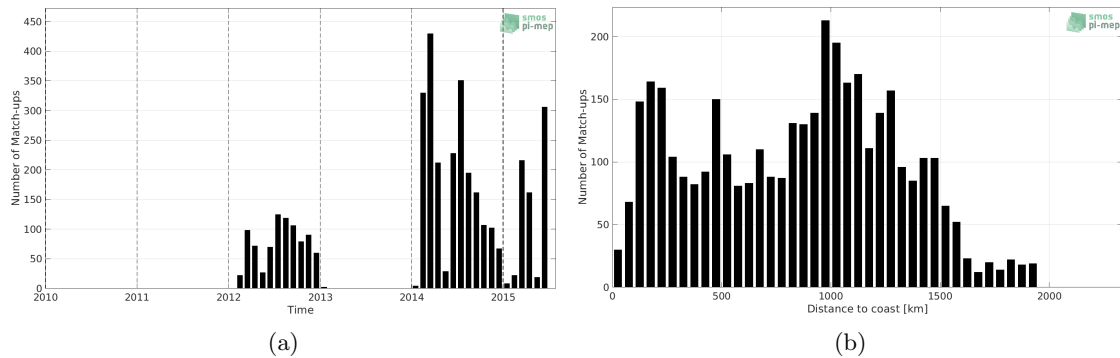
Figure 1: Number of match-ups between Sea mammals and Aquarius SSS L3 OR v5 - Monthly - Rain mask (NASA-GSFC) SSS as a function of time (a) and as function of the distance to coast (b) over the North Pacific Ocean Pi-MEP region and for the full satellite product period.
