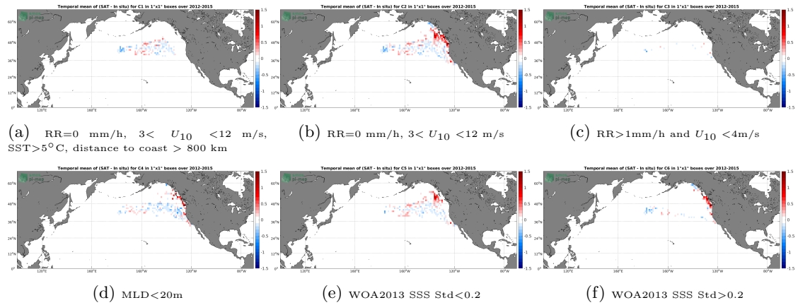
Figure 12: Temporal mean gridded over spatial boxes of size 1^{\circ}\times 1^{\circ} of \Delta\text{SSS} (Aquarius SSS L3 OR v5 - Monthly - Rain mask (NASA-GSFC) - Sea mammals) for 6 different subdatasets corresponding to:RR=0 mm/h, 3 < U_{10} < 12 m/s, SST >5^{\circ}\text{C} , distance to coast > 800 km (a), RR=0 mm/h, 3 < U_{10} < 12 m/s (b), RR >1 mm/h and U_{10} < 4 m/s (c),MLD <20 m (d),WOA2013 SSS Std <0.2 (e),WOA2013 SSS Std >0.2 (f).
