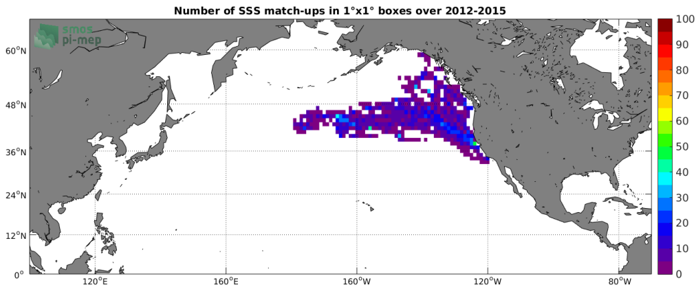
Figure 4: Number of SSS match-ups between Sea mammals SSS and the Aquarius-L3-OR-V5-MONTHLY-RAIN-MASK-1DEG SSS product for the North Pacific Ocean Pi-MEP region over 1°x1° boxes and for the full satellite product period.
