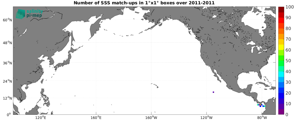
Figure 4: Number of SSS match-ups between Surface drifters SSS and the Aquarius SSS L3 OR v5 - Monthly - Rain mask (NASA-GSFC) SSS product for the North Pacific Ocean Pi-MEP region over 1^\circ \times 1^\circ boxes and for the full satellite product period.
