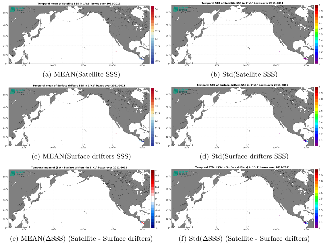
Figure 6: Temporal mean (left) and Std (right) of SSS from Aquarius SSS L3 OR v5 - Monthly - Rain mask (NASA-GSFC) (top), Surface drifters (middle), and of \Delta SSS (Satellite - Surface drifters). Only match-up pairs are used to generate these maps.
