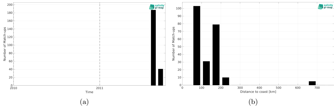
Figure 2: Number of match-ups between Surface drifters and Aquarius SSS L3 OR v5 - Monthly - Rain mask (NASA-GSFC) SSS as a function of time (a) and as function of the distance to coast (b) over the North Pacific Ocean Pi-MEP region and for the full satellite product period.
