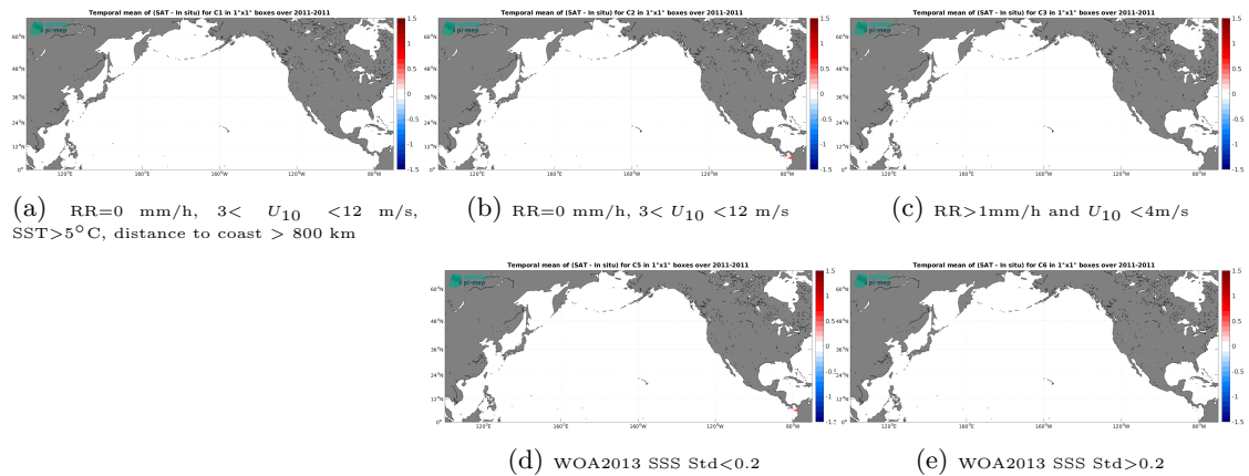
Figure 13: Temporal mean gridded over spatial boxes of size 1^\circ \times 1^\circ of \Delta\text{SSS} (Aquarius SSS L3 OR v5 - Monthly - Rain mask (NASA-GSFC) - Surface drifters) for 5 different subdatasets corresponding to:RR=0 mm/h, 3 < U_{10} < 12 m/s, SST >5^\circ\text{C} , distance to coast > 800 km (a), RR=0 mm/h, 3 < U_{10} < 12 m/s (b), RR >1 mm/h and U_{10} < 4 m/s (c), WOA2013 SSS Std <0.2 (d), WOA2013 SSS Std >0.2 (e).
