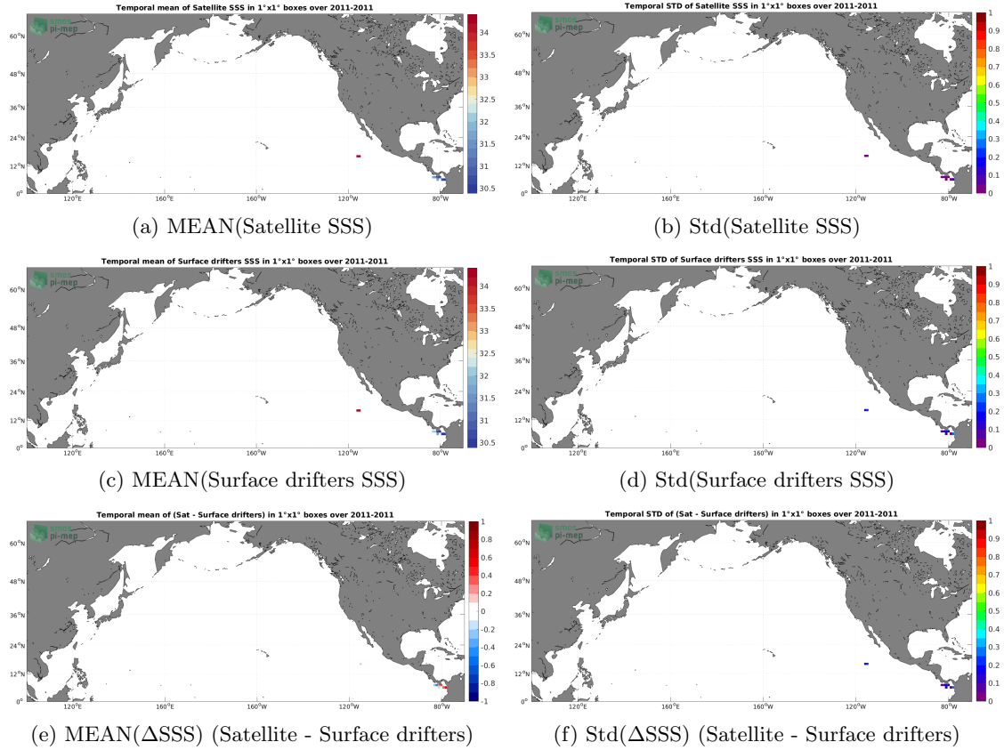
Figure 5: Temporal mean (left) and Std (right) of SSS from Aquarius SSS L3 OR v5 - Monthly - Rain mask (NASA-GSFC) (top), Surface drifters (middle), and of \Delta SSS (Satellite - Surface drifters). Only match-up pairs are used to generate these maps.
