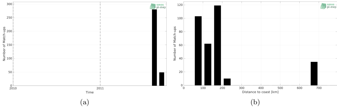
Figure 1: Number of match-ups between Surface drifters and Aquarius SSS L3 OR v5 - Monthly - Rain mask (NASA-GSFC) SSS as a function of time (a) and as function of the distance to coast (b) over the North Pacific Ocean Pi-MEP region and for the full satellite product period.
