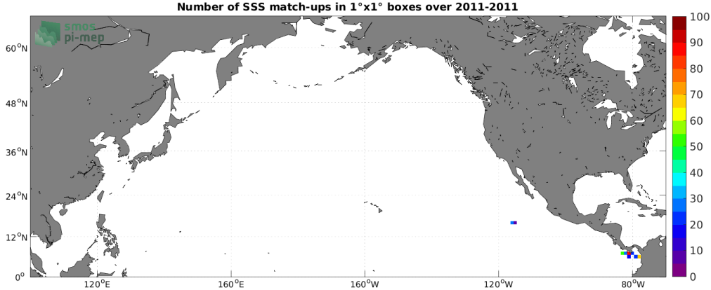
Figure 3: Number of SSS match-ups between Surface drifters SSS and the Aquarius SSS L3 OR v5 - Monthly - Rain mask (NASA-GSFC) SSS product for the North Pacific Ocean Pi-MEP region over 1^\circ \times 1^\circ boxes and for the full satellite product period.
