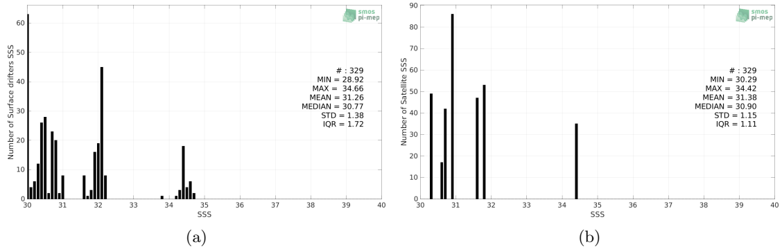
Figure 2: Histograms of SSS from Surface drifters (a) and Aquarius SSS L3 OR v5 - Monthly - Rain mask (NASA-GSFC) (b) considering all match-up pairs per bins of 0.1 over the North Pacific Ocean Pi-MEP region and for the full satellite product period.
