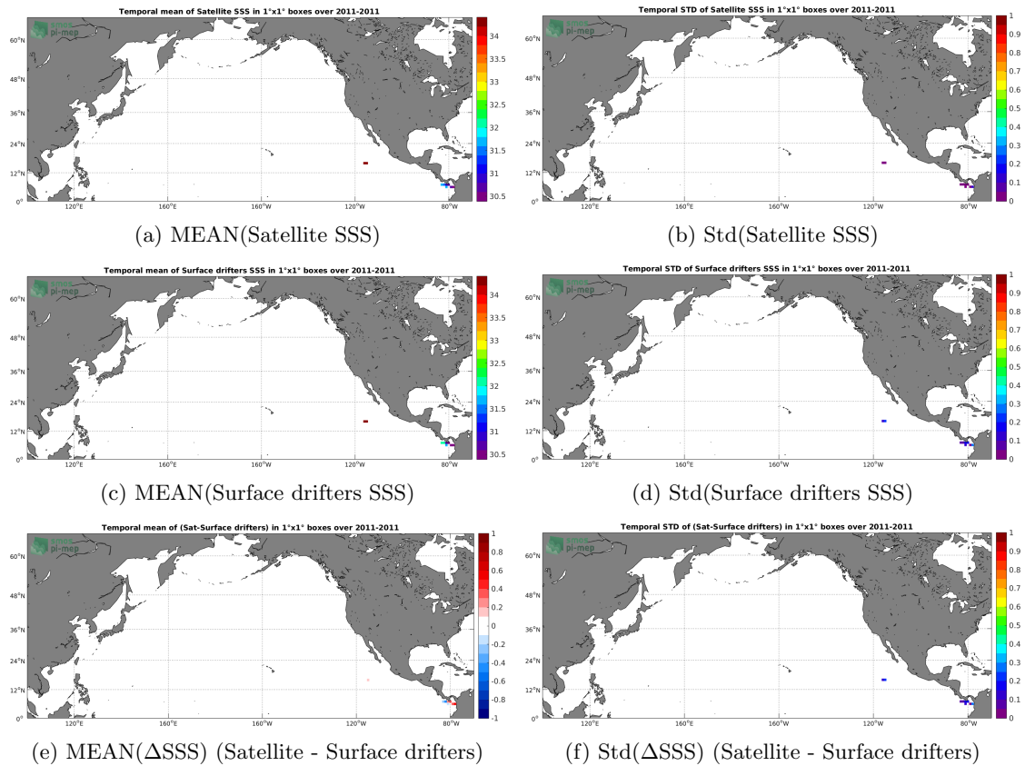
Figure 5: Temporal mean (left) and Std (right) of SSS from Aquarius-L3-OR-V5-MONTHLY-RAIN-MASK-1DEG (top), Surface drifters (middle), and of \Delta SSS (Satellite - Surface drifters). Only match-up pairs are used to generate these maps.
