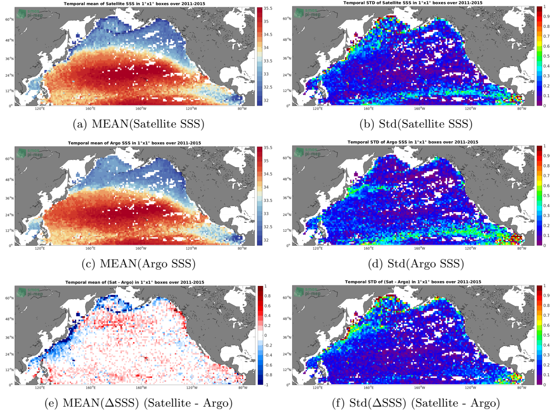
Figure 6: Temporal mean (left) and Std (right) of SSS from Aquarius SSS L3 OR v5 - Monthly - Rain mask (NASA-GSFC) (top), Argo (middle), and of \Delta\text{SSS} (Satellite - Argo). Only match-up pairs are used to generate these maps.
