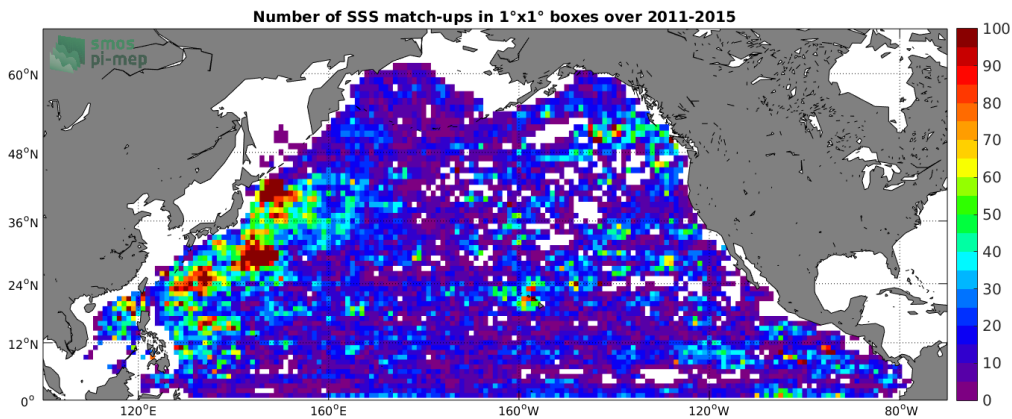
Figure 4: Number of SSS match-ups between Argo SSS and the Aquarius-L3-OR-V5-MONTHLY-RAIN-MASK-1DEG SSS product for the North Pacific Ocean Pi-MEP region over 1°x1° boxes and for the full satellite product period.
