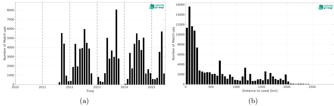
Figure 2: Number of match-ups between TSG (SAMOS) and Aquarius SSS L3 CAP v5 - 7-Day running (JPL) SSS as a function of time (a) and as function of the distance to coast (b) over the North Pacific Ocean Pi-MEP region and for the full satellite product period.
