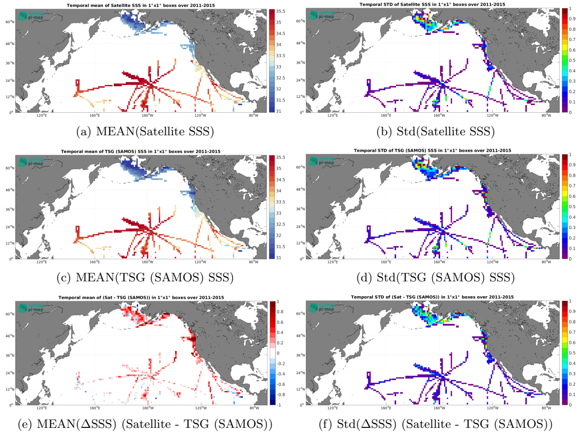
Figure 7: Temporal mean (left) and Std (right) of SSS from Aquarius SSS L3 CAP v5 - 7-Day running (JPL) (top), TSG (SAMOS) (middle), and of \Delta SSS (Satellite - TSG (SAMOS)). Only match-up pairs are used to generate these maps.
