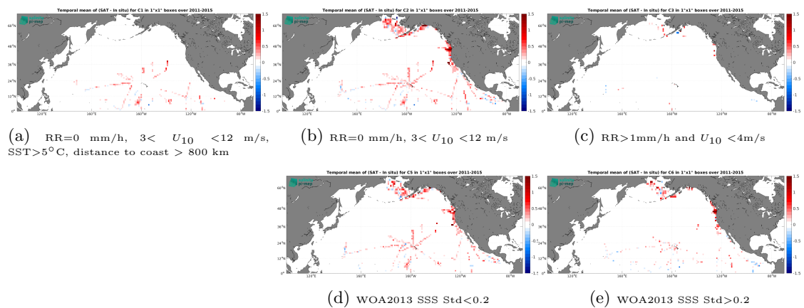
Figure 14: Temporal mean gridded over spatial boxes of size 1^\circ \times 1^\circ of \Delta\text{SSS} (Aquarius SSS L3 CAP v5 - 7-Day running (JPL) - TSG (SAMOS)) for 5 different subdatasets corresponding to: RR=0 mm/h, 3 < U_{10} < 12 m/s, SST > 5°C, distance to coast > 800 km (a), RR=0 mm/h, 3 < U_{10} < 12 m/s (b), RR > 1 mm/h and U_{10} < 4 m/s (c), WOA2013 SSS Std < 0.2 (d), WOA2013 SSS Std > 0.2 (e).
