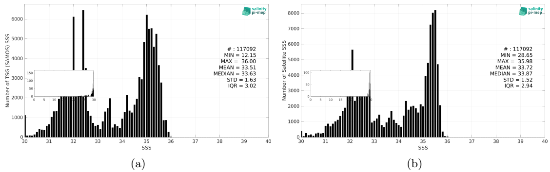
Figure 3: Histograms of SSS from TSG (SAMOS) (a) and Aquarius SSS L3 CAP v5 - 7-Day running (JPL) (b) considering all match-up pairs per bins of 0.1 over the North Pacific Ocean Pi-MEP region and for the full satellite product period.
