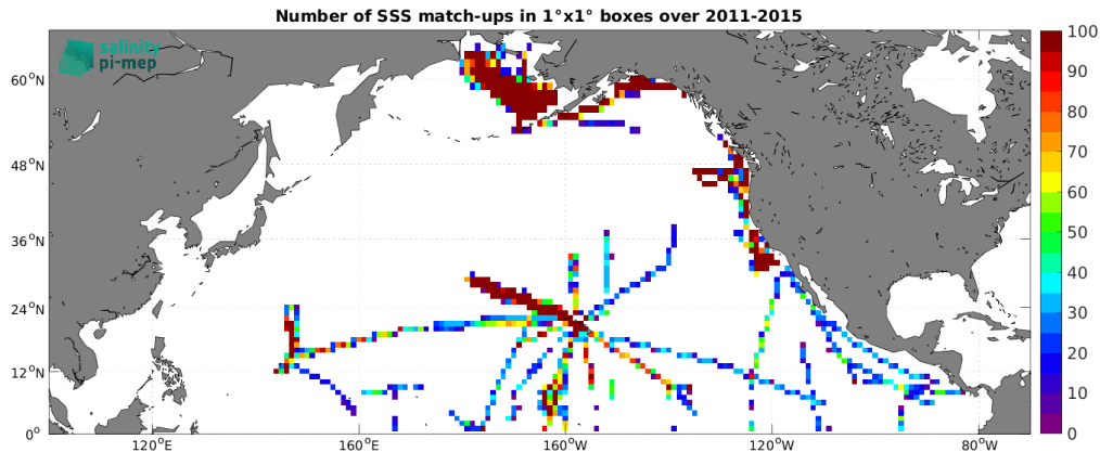
Figure 5: Number of SSS match-ups between TSG (SAMOS) SSS and the Aquarius SSS L3 CAP v5 - 7-Day running (JPL) SSS product for the North Pacific Ocean Pi-MEP region over 1^\circ \times 1^\circ boxes and for the full satellite product period.
