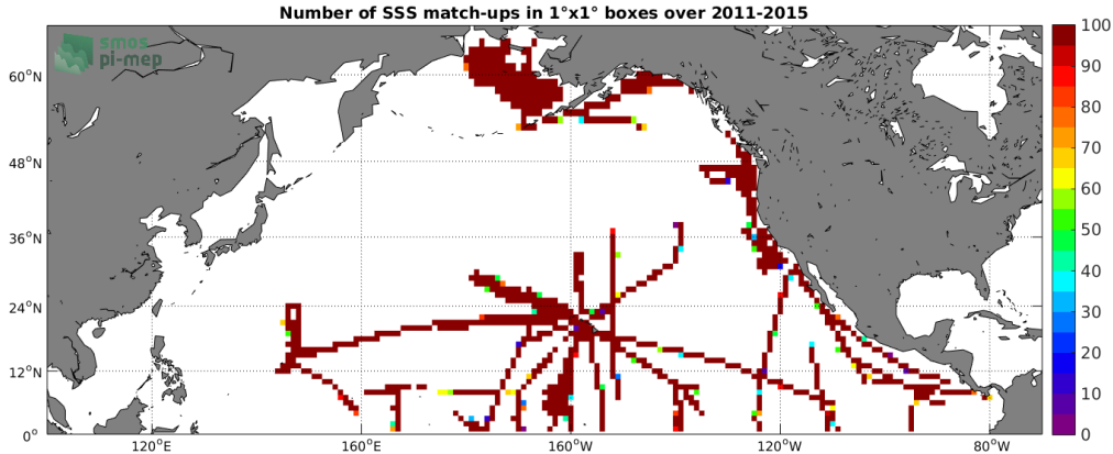
Figure 4: Number of SSS match-ups between TSG-SAMOS SSS and the Aquarius-L3-JPL-V5-7DAY-RUNNING SSS product for the North Pacific Ocean Pi-MEP region over 1°x1° boxes and for the full satellite product period.
