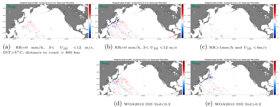
Figure 12: Temporal mean gridded over spatial boxes of size 1^\circ \times 1^\circ of \Delta\text{SSS} (Aquarius SSS L3 CAP v5 - 7-Day running (JPL) - TSG (LEGOS-DM)) for 5 different subdatasets corresponding to:RR=0 mm/h, 3 < U_{10} < 12 m/s, SST >5^\circ\text{C} , distance to coast > 800 km (a), RR=0 mm/h, 3 < U_{10} < 12 m/s (b), RR >1 mm/h and U_{10} < 4 m/s (c), WOA2013 SSS Std <0.2 (d), WOA2013 SSS Std >0.2 (e).
