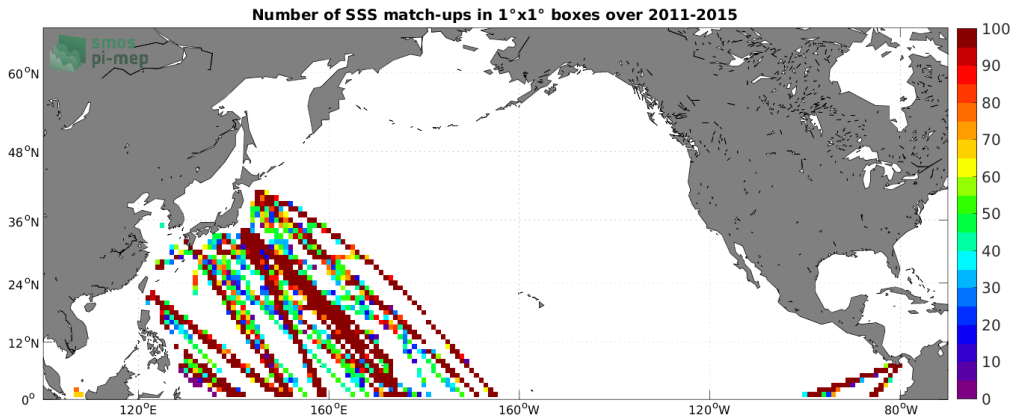
Figure 4: Number of SSS match-ups between TSG (LEGOS-DM) SSS and the Aquarius SSS L3 CAP v5 - 7-Day running (JPL) SSS product for the North Pacific Ocean Pi-MEP region over 1^\circ \times 1^\circ boxes and for the full satellite product period.
