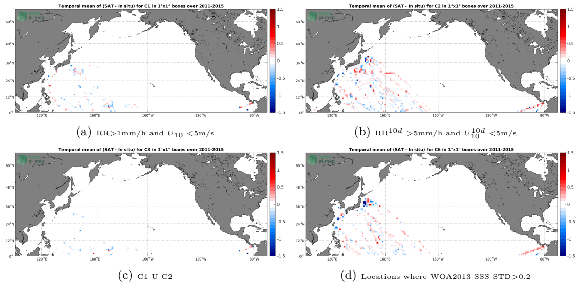
Figure 12: Temporal mean gridded over spatial boxes of size 1^\circ \times 1^\circ of \Delta SSS (Aquarius-L3-JPL-V5-7DAY-RUNNING - TSG-LEGOS-DM) for 4 different subdatasets corresponding to: RR > 1\text{mm/h} and U_{10} < 5\text{m/s} (a), RR^{10d} > 5\text{mm/h} and U_{10}^{10d} < 5\text{m/s} (b), C1 U C2 (c), Locations where WOA2013 SSS STD > 0.2 (d).
