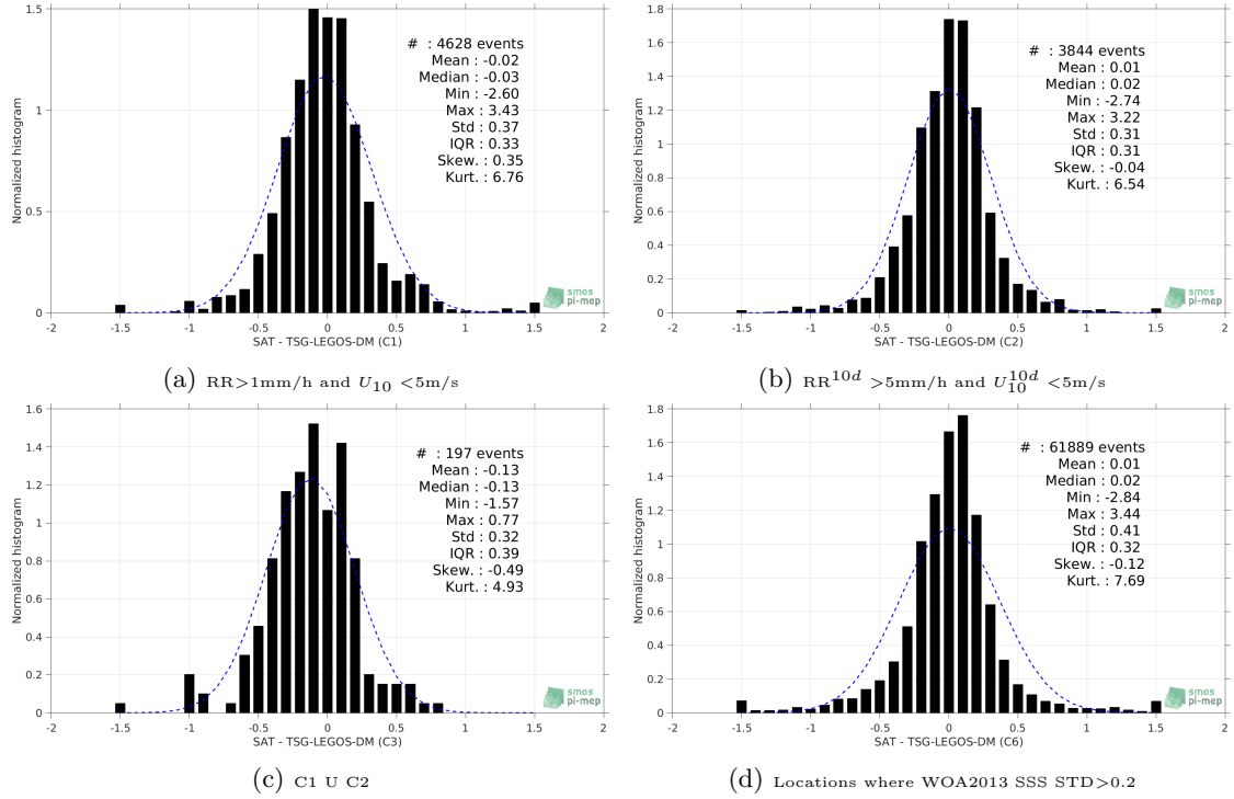
Figure 13: Normalized histogram of \Delta SSS (Aquarius-L3-JPL-V5-7DAY-RUNNING - TSG-LEGOS-DM) for 6 different subdatasets corresponding to: RR > 1mm/h and U_{10} < 5 m/s (a), RR^{10d} > 5 mm/h and U_{10}^{10d} < 5 m/s (b), C1 U C2 (c), Locations where WOA2013 SSS STD > 0.2 (d).
