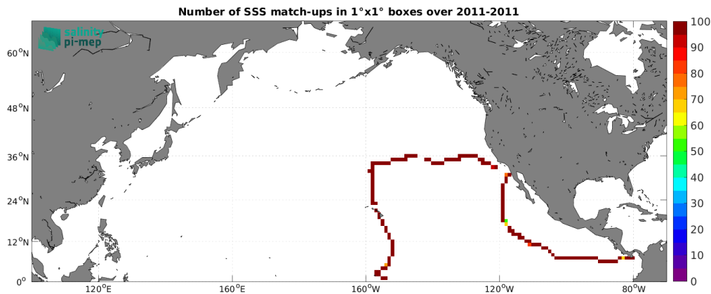
Figure 4: Number of SSS match-ups between TSG (GOSUD-Sailing-ship) SSS and the Aquarius SSS L3 CAP v5 - 7-Day running (JPL) SSS product for the North Pacific Ocean Pi-MEP region over 1^\circ \times 1^\circ boxes and for the full satellite product period.
