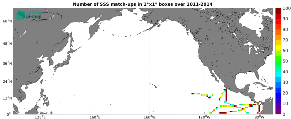
Figure 5: Number of SSS match-ups between TSG (GOSUD-Research-vessel) SSS and the Aquarius SSS L3 CAP v5 - 7-Day running (JPL) SSS product for the North Pacific Ocean Pi-MEP region over 1^\circ \times 1^\circ boxes and for the full satellite product period.
