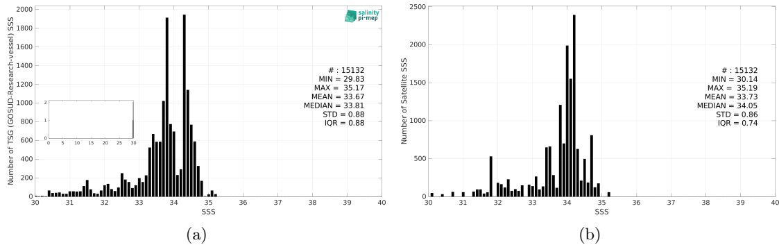
Figure 3: Histograms of SSS from TSG (GOSUD-Research-vessel) (a) and Aquarius SSS L3 CAP v5 - 7-Day running (JPL) (b) considering all match-up pairs per bins of 0.1 over the North Pacific Ocean Pi-MEP region and for the full satellite product period.
