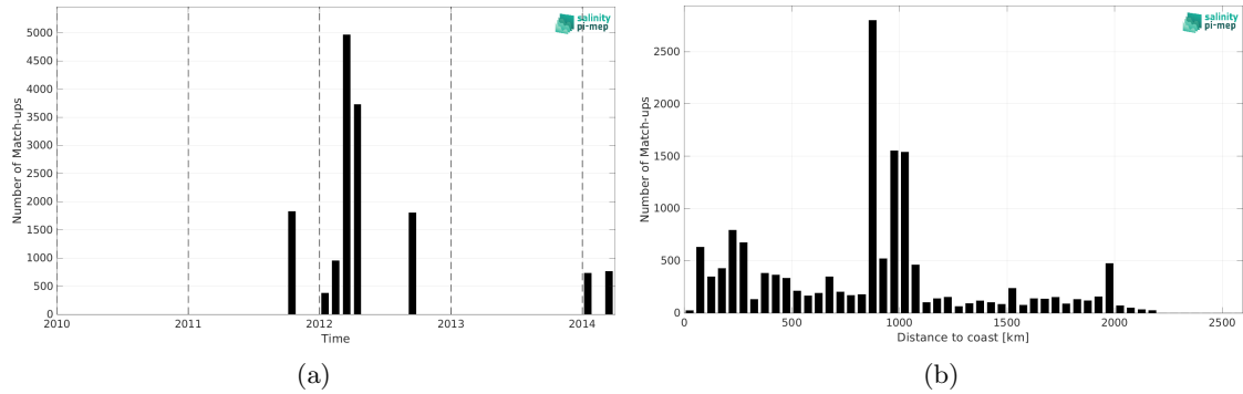
Figure 2: Number of match-ups between TSG (GOSUD-Research-vessel) and Aquarius SSS L3 CAP v5 - 7-Day running (JPL) SSS as a function of time (a) and as function of the distance to coast (b) over the North Pacific Ocean Pi-MEP region and for the full satellite product period.
