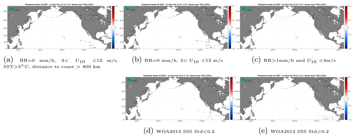
Figure 12: Temporal mean gridded over spatial boxes of size 1^\circ \times 1^\circ of \Delta\text{SSS} (Aquarius SSS L3 CAP v5 - 7-Day running (JPL) - TSG (GOSUD-Research-vessel)) for 5 different subdatasets corresponding to: RR=0 mm/h, 3 < U_{10} < 12 m/s, SST > 5°C, distance to coast > 800 km (a), RR=0 mm/h, 3 < U_{10} < 12 m/s (b), RR > 1mm/h and U_{10} < 4 m/s (c), WOA2013 SSS Std < 0.2 (d), WOA2013 SSS Std > 0.2 (e).
