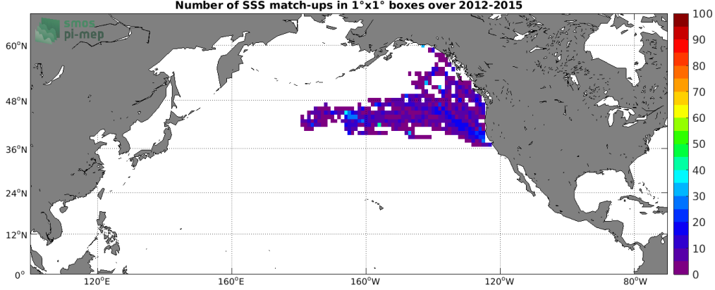
Figure 4: Number of SSS match-ups between Sea mammals SSS and the Aquarius SSS L3 CAP v5 - 7-Day running (JPL) SSS product for the North Pacific Ocean Pi-MEP region over 1^\circ \times 1^\circ boxes and for the full satellite product period.
