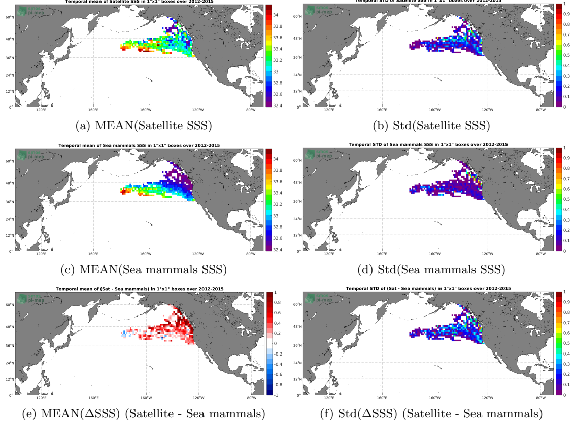
Figure 6: Temporal mean (left) and Std (right) of SSS from Aquarius SSS L3 CAP v5 - 7-Day running (JPL) (top), Sea mammals (middle), and of \Delta SSS (Satellite - Sea mammals). Only match-up pairs are used to generate these maps.
