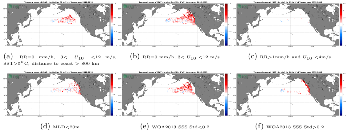
Figure 12: Temporal mean gridded over spatial boxes of size 1^\circ \times 1^\circ of \Delta SSS (Aquarius SSS L3 CAP v5 - 7-Day running (JPL) - Sea mammals) for 6 different subdatasets corresponding to: RR=0 mm/h, 3 < U_{10} < 12 m/s, SST > 5^\circ C , distance to coast > 800 km (a), RR=0 mm/h, 3 < U_{10} < 12 m/s (b), RR > 1 mm/h and U_{10} < 4 m/s (c), MLD < 20 m (d), WOA2013 SSS Std < 0.2 (e), WOA2013 SSS Std > 0.2 (f).
