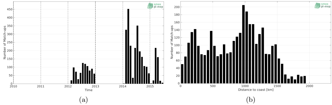
Figure 1: Number of match-ups between Sea mammals and Aquarius SSS L3 CAP v5 - 7-Day running (JPL) SSS as a function of time (a) and as function of the distance to coast (b) over the North Pacific Ocean Pi-MEP region and for the full satellite product period.
