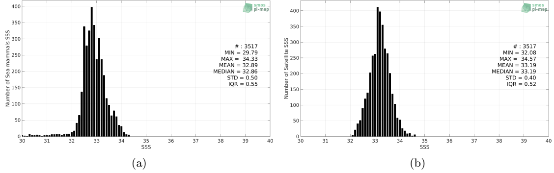
Figure 2: Histograms of SSS from Sea mammals (a) and Aquarius SSS L3 CAP v5 - 7-Day running (JPL) (b) considering all match-up pairs per bins of 0.1 over the North Pacific Ocean Pi-MEP region and for the full satellite product period.
