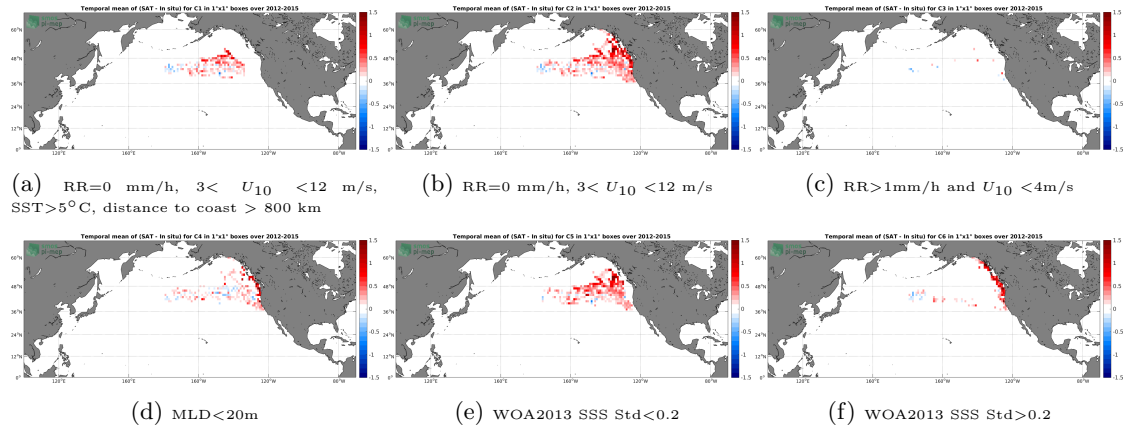
Figure 12: Temporal mean gridded over spatial boxes of size 1^\circ \times 1^\circ of \Delta SSS (Aquarius-L3-JPL-V5-7DAY-RUNNING - Sea mammals) for 6 different subdatasets corresponding to: RR=0 mm/h, 3 < U_{10} < 12 m/s, SST > 5^\circ\text{C} , distance to coast > 800 km (a), RR=0 mm/h, 3 < U_{10} < 12 m/s (b), RR > 1 mm/h and U_{10} < 4 m/s (c), MLD < 20 m (d), WOA2013 SSS Std < 0.2 (e), WOA2013 SSS Std > 0.2 (f).
