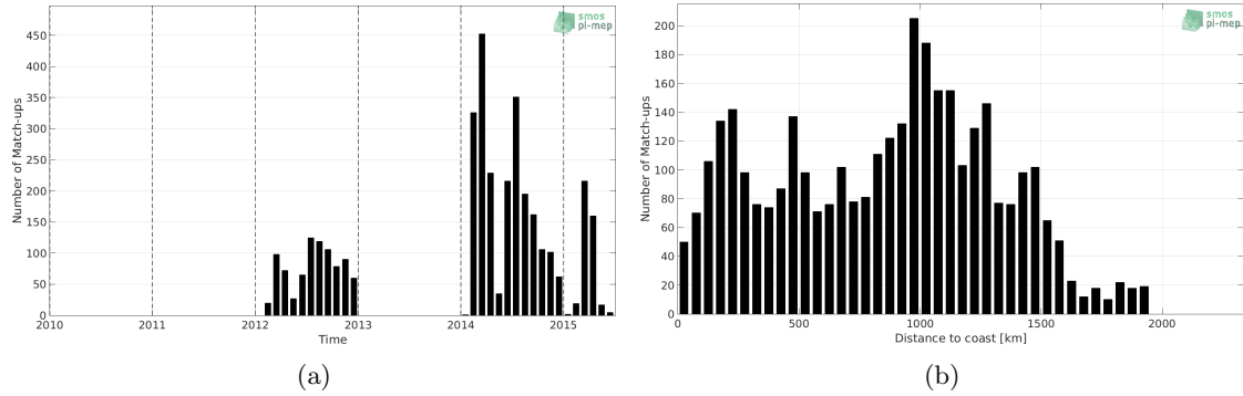
Figure 1: Number of match-ups between Sea mammals and Aquarius-L3-JPL-V5-7DAY-RUNNING SSS as a function of time (a) and as function of the distance to coast (b) over the North Pacific Ocean Pi-MEP region and for the full satellite product period.
