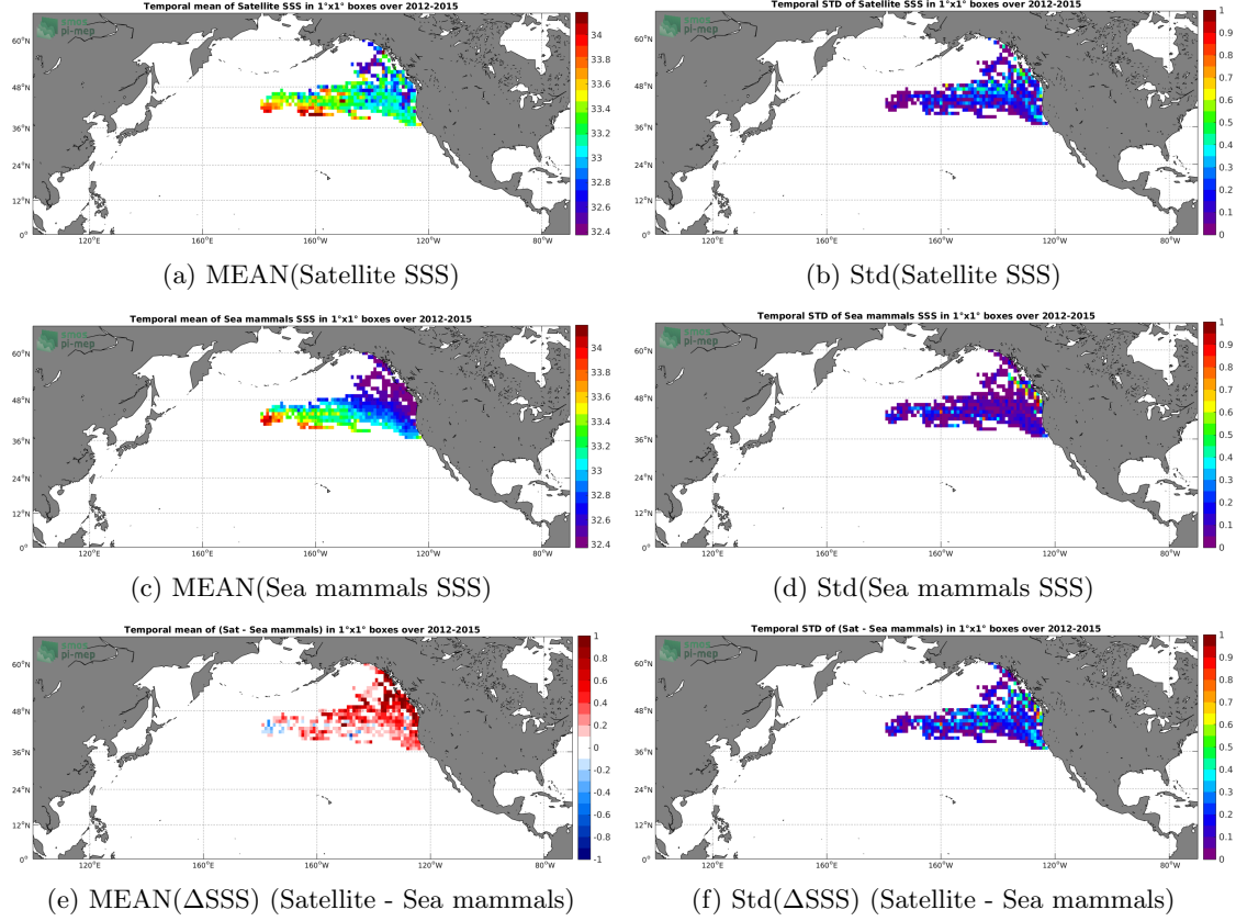
Figure 6: Temporal mean (left) and Std (right) of SSS from Aquarius-L3-JPL-V5-7DAY-RUNNING (top), Sea mammals in situ dataset (middle), and of \Delta SSS (Satellite - Sea mammals). Only match-up pairs are used to generate these maps.
