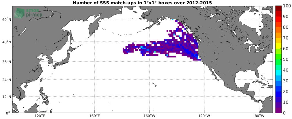
Figure 4: Number of SSS match-ups between Sea mammals SSS and the Aquarius-L3-JPL-V5-7DAY-RUNNING SSS product for the North Pacific Ocean Pi-MEP region over 1^\circ \times 1^\circ boxes and for the full satellite product period.
