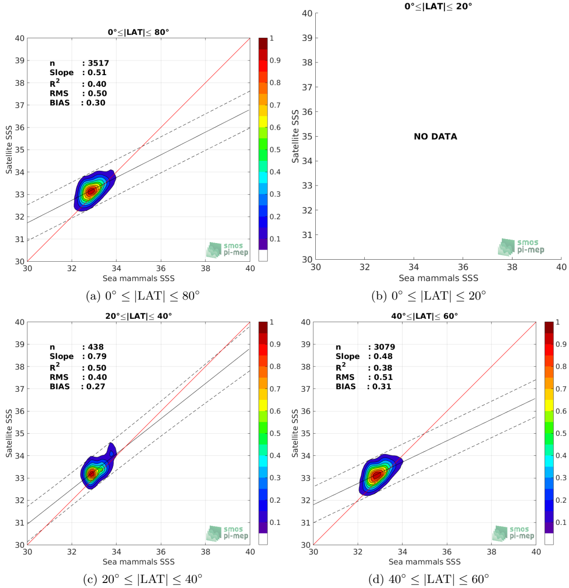
Figure 9: Contour maps of the concentration of Aquarius-L3-JPL-V5-7DAY-RUNNING SSS (y-axis) versus Sea mammals SSS (x-axis) at match-up pairs for different latitude bands. For each plot, the red line shows x=y . The black thin and dashed lines indicate a linear fit through the data cloud and the \pm 95\% confidence levels, respectively. The number match-up pairs n , the slope and R^2 coefficient of the linear fit, the root mean square (RMS) and the mean bias between satellite and in situ data are indicated for each latitude band in each plots.
