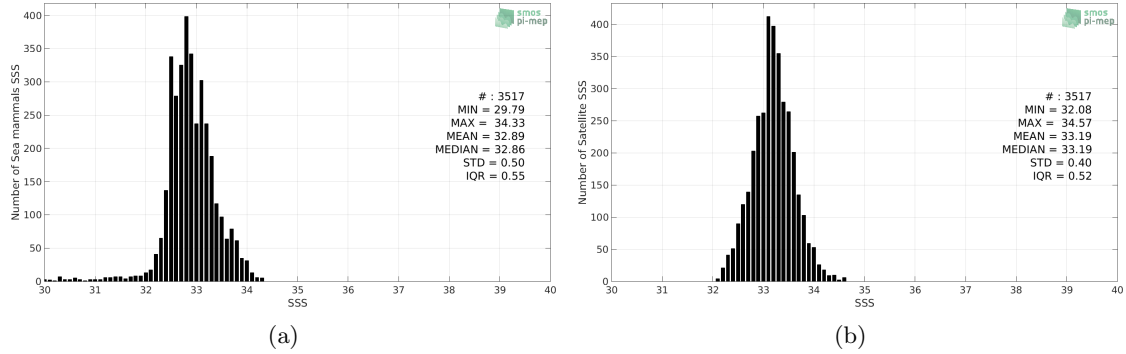
Figure 2: Histograms of SSS from Sea mammals (a) and Aquarius-L3-JPL-V5-7DAY-RUNNING (b) considering all match-up pairs per bins of 0.1 over the North Pacific Ocean Pi-MEP region and for the full satellite product period.
