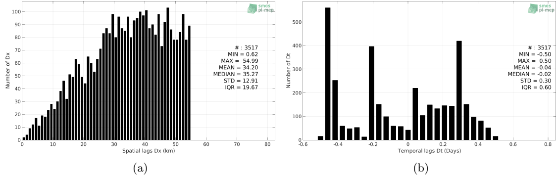
Figure 5: Histograms of the spatial (a) and temporal (b) lags between the time of the Sea mammals measurements and the date of the corresponding Aquarius-L3-JPL-V5-7DAY-RUNNING SSS product.
