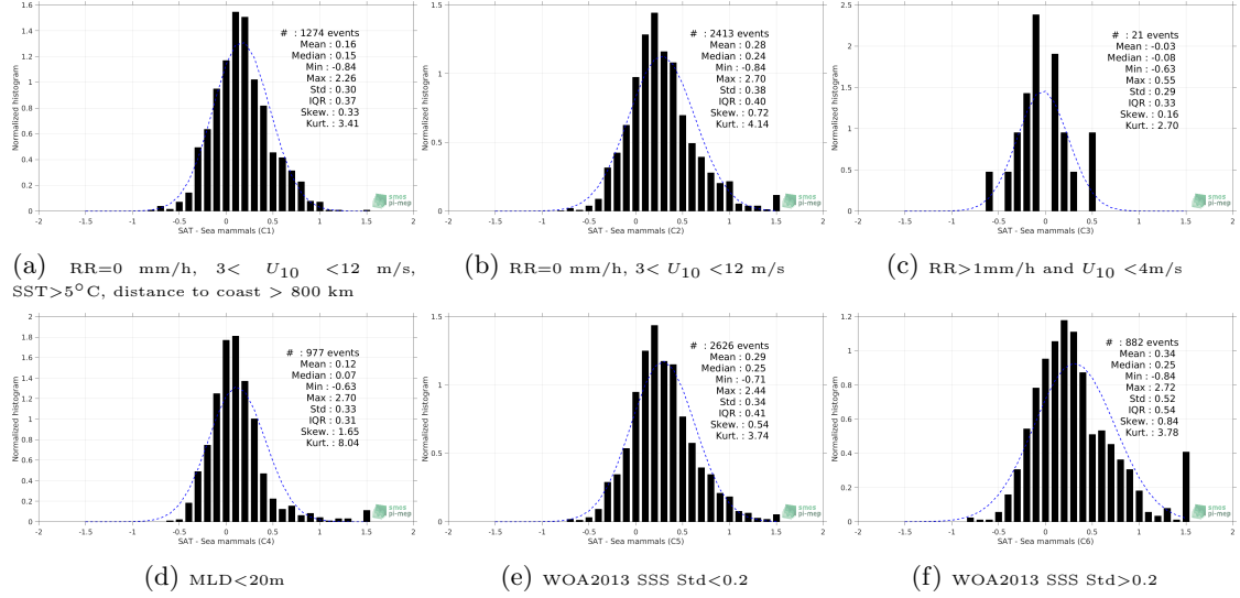
Figure 13: Normalized histogram of \Delta SSS (Aquarius-L3-JPL-V5-7DAY-RUNNING - Sea mammals) for 6 different subdatasets corresponding to: RR=0 mm/h, 3 < U_{10} < 12 m/s, SST>5°C, distance to coast > 800 km (a), RR=0 mm/h, 3 < U_{10} < 12 m/s (b), RR>1mm/h and U_{10} < 4 m/s (c), MLD<20m (d), WOA2013 SSS Std<0.2 (e), WOA2013 SSS Std>0.2 (f).
