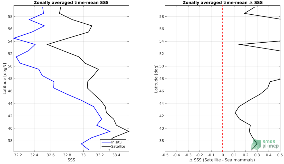
Figure 8: Left panel: Zonal mean SSS from Aquarius-L3-JPL-V5-7DAY-RUNNING satellite product (black) and from Sea mammals (blue). Right panel: Zonal mean of \Delta SSS (Satellite - Sea mammals) for all the collected Pi-MEP match-up pairs estimated over the full satellite product period.
