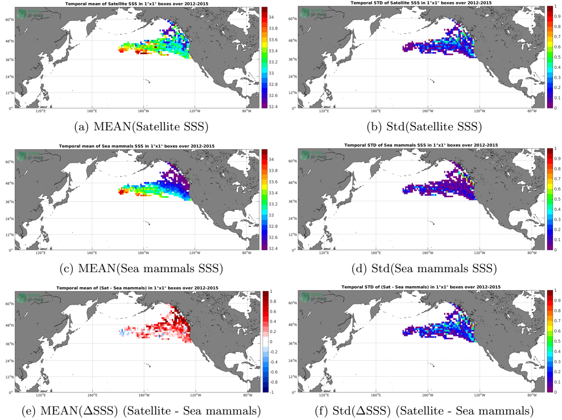
Figure 6: Temporal mean (left) and Std (right) of SSS from Aquarius-L3-JPL-V5-7DAY-RUNNING (top), Sea mammals (middle), and of \Delta SSS (Satellite - Sea mammals). Only match-up pairs are used to generate these maps.
