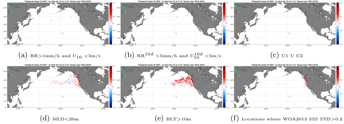
Figure 12: Temporal mean gridded over spatial boxes of size 1^\circ \times 1^\circ of \Delta SSS (Aquarius-L3-JPL-V5-7DAY-RUNNING - Sea mammals) for 6 different subdatasets corresponding to: RR > 1\text{mm/h} and U_{10} < 5\text{m/s} (a), RR^{10d} > 5\text{mm/h} and U_{10}^{10d} < 5\text{m/s} (b), C1 U C2 (c), MLD < 20\text{m} (d), BLT > 10\text{m} (e), Locations where WOA2013 SSS STD > 0.2 (f).
