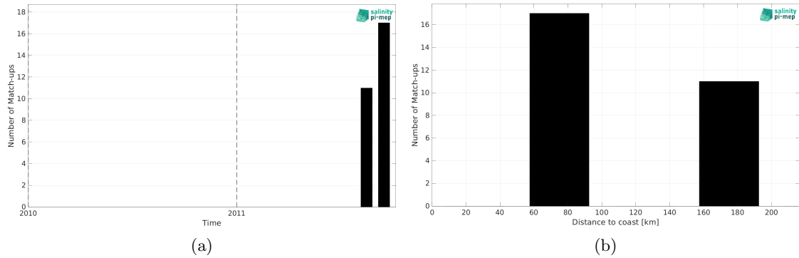
Figure 2: Number of match-ups between Surface drifters and Aquarius SSS L3 CAP v5 - 7-Day running (JPL) SSS as a function of time (a) and as function of the distance to coast (b) over the North Pacific Ocean Pi-MEP region and for the full satellite product period.
