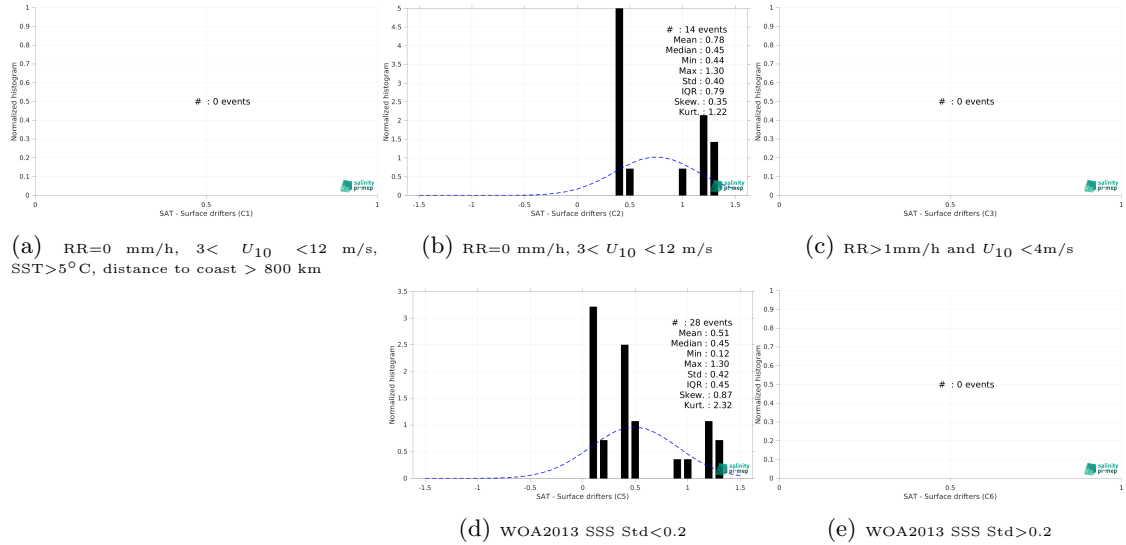
Figure 14: Normalized histogram of \Delta SSS (Aquarius SSS L3 CAP v5 - 7-Day running (JPL) - Surface drifters) for 5 different subdatasets corresponding to: RR=0 mm/h, 3 < U_{10} < 12 m/s, SST > 5°C, distance to coast > 800 km (a), RR=0 mm/h, 3 < U_{10} < 12 m/s (b), RR > 1mm/h and U_{10} < 4 m/s (c), WOA2013 SSS Std < 0.2 (d), WOA2013 SSS Std > 0.2 (e).
