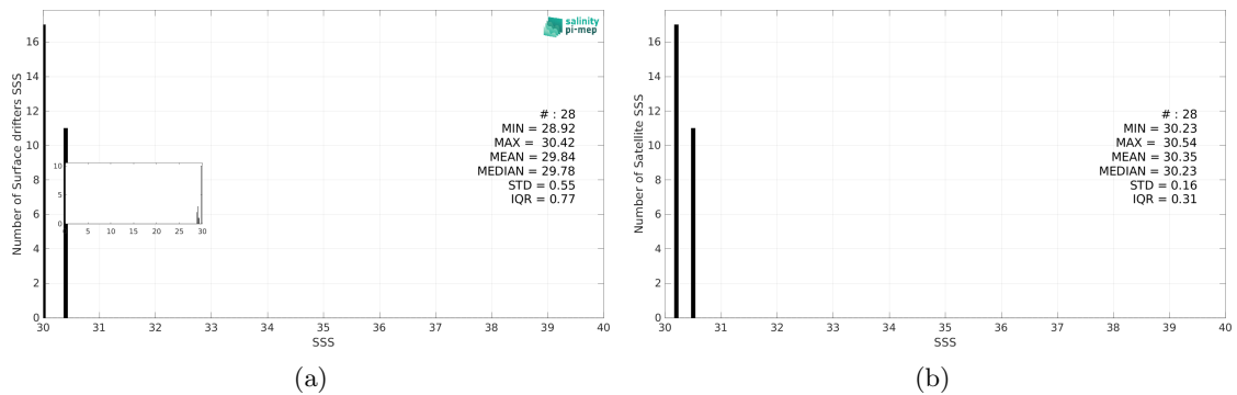
Figure 3: Histograms of SSS from Surface drifters (a) and Aquarius SSS L3 CAP v5 - 7-Day running (JPL) (b) considering all match-up pairs per bins of 0.1 over the North Pacific Ocean Pi-MEP region and for the full satellite product period.
