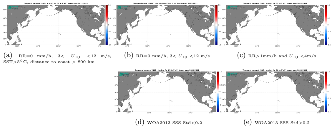
Figure 13: Temporal mean gridded over spatial boxes of size 1^\circ \times 1^\circ of \Delta\text{SSS} (Aquarius SSS L3 CAP v5 - 7-Day running (JPL) - Surface drifters) for 5 different subdatasets corresponding to:RR=0 mm/h, 3 < U_{10} < 12 m/s, SST >5^\circ\text{C} , distance to coast > 800 km (a), RR=0 mm/h, 3 < U_{10} < 12 m/s (b), RR >1 mm/h and U_{10} < 4 m/s (c), WOA2013 SSS Std <0.2 (d), WOA2013 SSS Std >0.2 (e).
