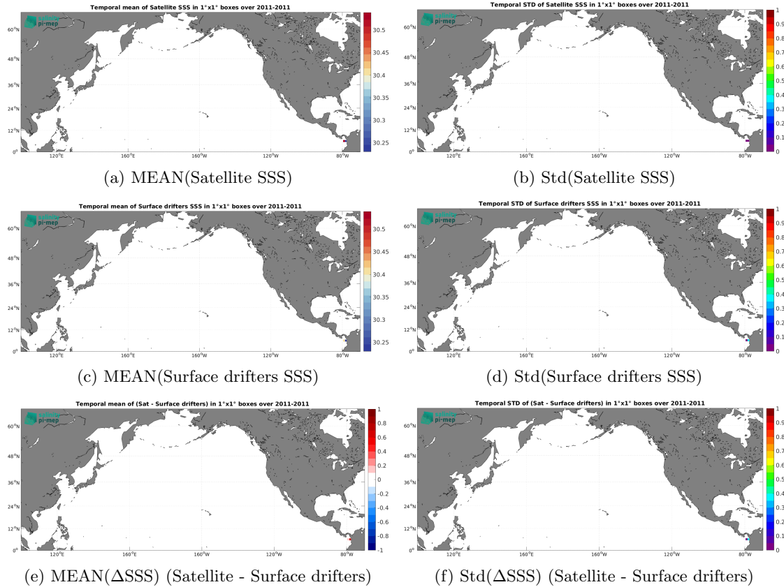
Figure 6: Temporal mean (left) and Std (right) of SSS from Aquarius SSS L3 CAP v5 - 7-Day running (JPL) (top), Surface drifters (middle), and of \Delta SSS (Satellite - Surface drifters). Only match-up pairs are used to generate these maps.
