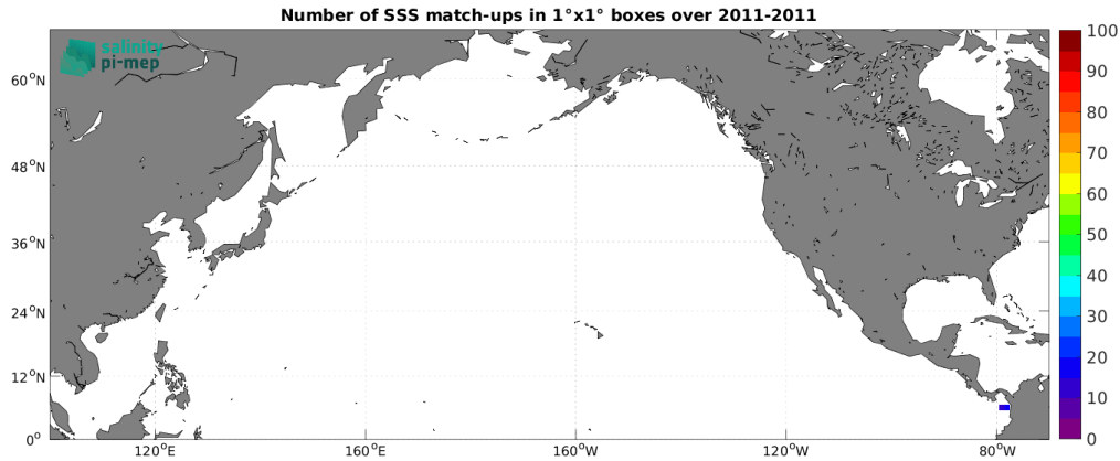
Figure 4: Number of SSS match-ups between Surface drifters SSS and the Aquarius SSS L3 CAP v5 - 7-Day running (JPL) SSS product for the North Pacific Ocean Pi-MEP region over 1^\circ \times 1^\circ boxes and for the full satellite product period.
