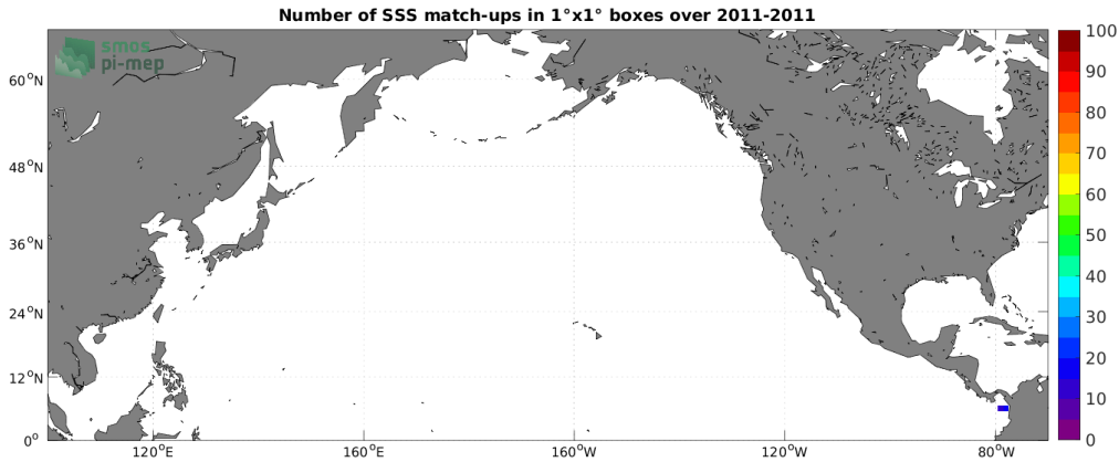
Figure 3: Number of SSS match-ups between Surface drifters SSS and the Aquarius SSS L3 CAP v5 - 7-Day running (JPL) SSS product for the North Pacific Ocean Pi-MEP region over 1^\circ \times 1^\circ boxes and for the full satellite product period.
