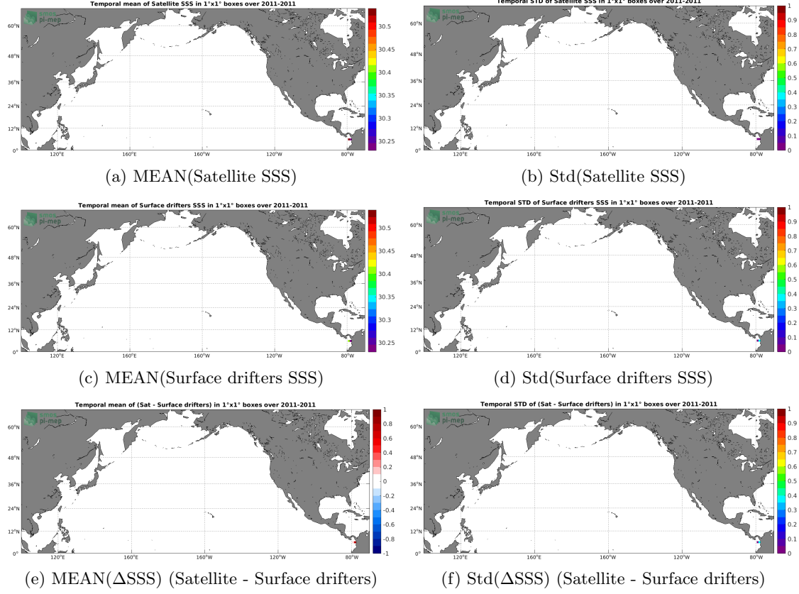
Figure 5: Temporal mean (left) and Std (right) of SSS from Aquarius SSS L3 CAP v5 - 7-Day running (JPL) (top), Surface drifters (middle), and of \Delta SSS (Satellite - Surface drifters). Only match-up pairs are used to generate these maps.
