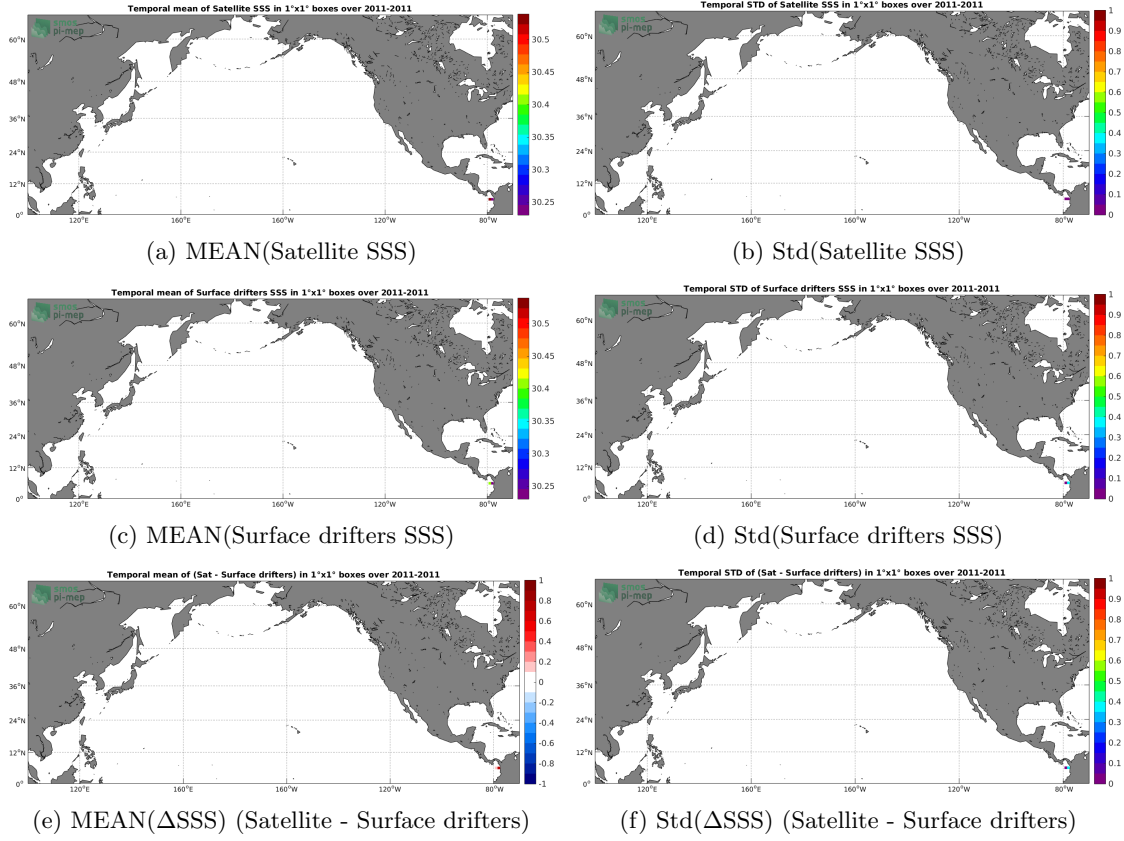
Figure 5: Temporal mean (left) and Std (right) of SSS from Aquarius-L3-JPL-V5-7DAY-RUNNING (top), Surface drifters (middle), and of \Delta SSS (Satellite - Surface drifters). Only match-up pairs are used to generate these maps.
