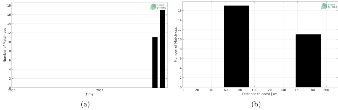
Figure 1: Number of match-ups between Surface drifters and Aquarius-L3-JPL-V5-7DAY-RUNNING SSS as a function of time (a) and as function of the distance to coast (b) over the North Pacific Ocean Pi-MEP region and for the full satellite product period.
