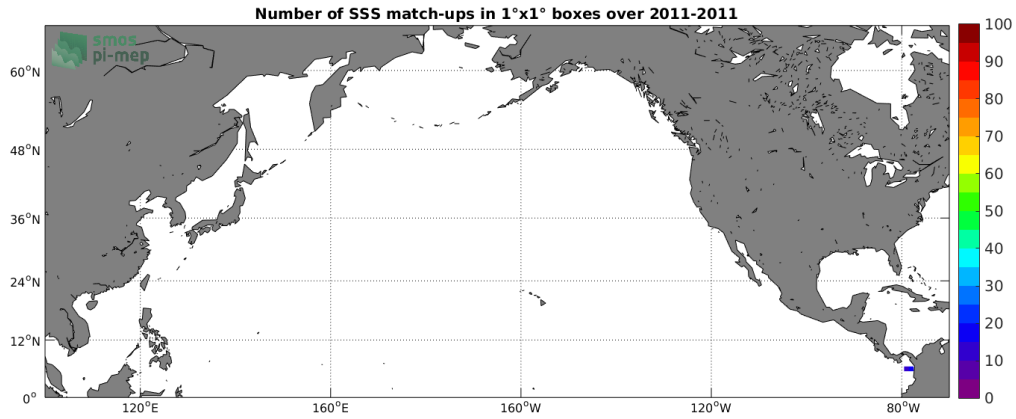
Figure 3: Number of SSS match-ups between Surface drifters SSS and the Aquarius-L3-JPL-V5-7DAY-RUNNING SSS product for the North Pacific Ocean Pi-MEP region over 1^\circ \times 1^\circ boxes and for the full satellite product period.
