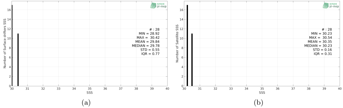
Figure 2: Histograms of SSS from Surface drifters (a) and Aquarius-L3-JPL-V5-7DAY-RUNNING (b) considering all match-up pairs per bins of 0.1 over the North Pacific Ocean Pi-MEP region and for the full satellite product period.
