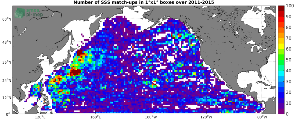
Figure 4: Number of SSS match-ups between Argo SSS and the Aquarius-L3-JPL-V5-7DAY-RUNNING SSS product for the North Pacific Ocean Pi-MEP region over 1^\circ \times 1^\circ boxes and for the full satellite product period.
