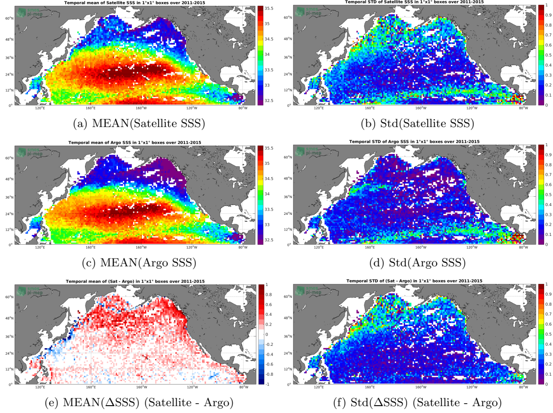
Figure 6: Temporal mean (left) and Std (right) of SSS from Aquarius-L3-JPL-V5-7DAY-RUNNING (top), Argo (middle), and of \Delta\text{SSS} (Satellite - Argo). Only match-up pairs are used to generate these maps.
