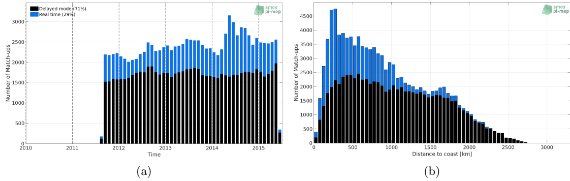
Figure 1: Number of match-ups between Argo and Aquarius-L3-JPL-V5-7DAY-RUNNING SSS as a function of time (a) and as function of the distance to coast (b) over the North Pacific Ocean Pi-MEP region and for the full satellite product period.
