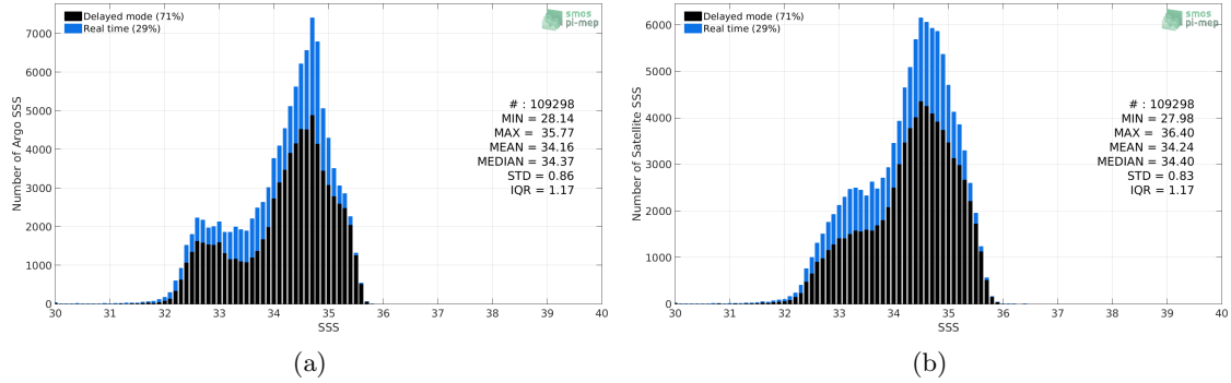
Figure 2: Histograms of SSS from Argo (a) and Aquarius-L3-JPL-V5-7DAY-RUNNING (b) considering all match-up pairs per bins of 0.1 over the North Pacific Ocean Pi-MEP region and for the full satellite product period.
