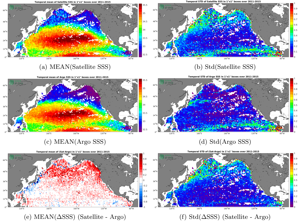
Figure 6: Temporal mean (left) and Std (right) of SSS from Aquarius-L3-JPL-V5-7DAY-RUNNING (top), Argo (middle), and of \Delta SSS (Satellite - Argo). Only match-up pairs are used to generate these maps.
