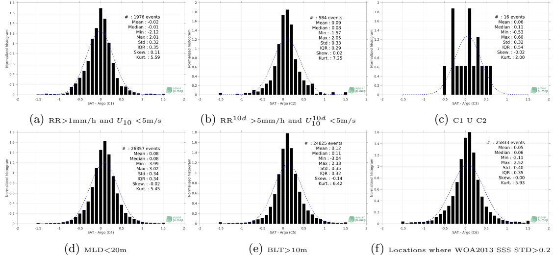
Figure 13: Normalized histogram of \Delta\text{SSS} (Aquarius-L3-JPL-V5-7DAY-RUNNING - Argo) for 6 different subdatasets corresponding to: RR > 1\text{mm/h} and U_{10} < 5\text{m/s} (a), RR^{10d} > 5\text{mm/h} and U_{10}^{10d} < 5\text{m/s} (b), C1 U C2 (c), MLD < 20\text{m} (d), BLT > 10\text{m} (e), Locations where WOA2013 SSS STD > 0.2 (f).
