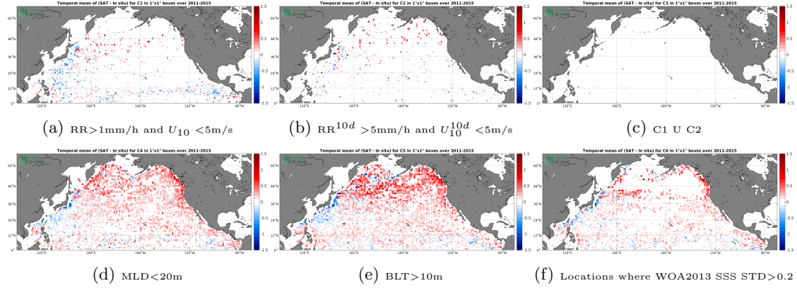
Figure 12: Temporal mean gridded over spatial boxes of size 1^\circ \times 1^\circ of \Delta\text{SSS} (Aquarius-L3-JPL-V5-7DAY-RUNNING - Argo) for 6 different subdatasets corresponding to: RR > 1\text{mm/h} and U_{10} < 5\text{m/s} (a), RR^{10d} > 5\text{mm/h} and U_{10}^{10d} < 5\text{m/s} (b), C1 U C2 (c), MLD < 20\text{m} (d), BLT > 10\text{m} (e), Locations where WOA2013 SSS STD > 0.2 (f).
