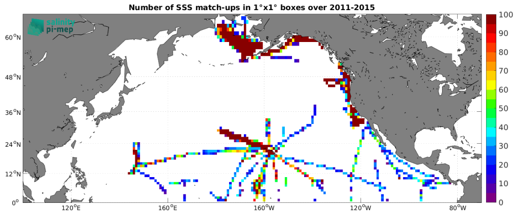
Figure 5: Number of SSS match-ups between TSG (SAMOS) SSS and the Aquarius SSS L3 CAP v5 - Monthly (JPL) SSS product for the North Pacific Ocean Pi-MEP region over 1^\circ \times 1^\circ boxes and for the full satellite product period.
