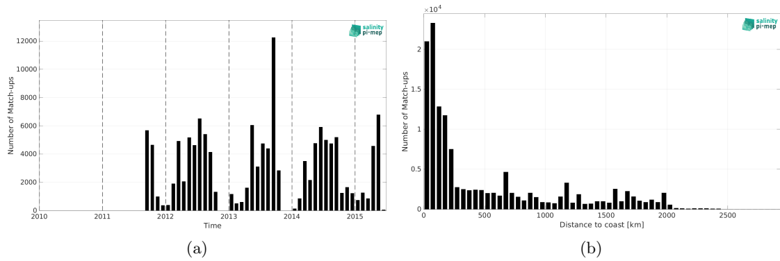
Figure 2: Number of match-ups between TSG (SAMOS) and Aquarius SSS L3 CAP v5 - Monthly (JPL) SSS as a function of time (a) and as function of the distance to coast (b) over the North Pacific Ocean Pi-MEP region and for the full satellite product period.
