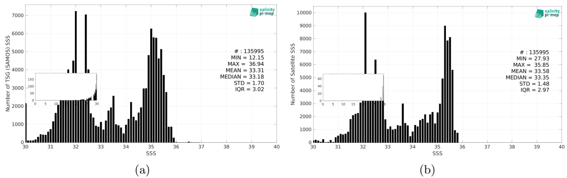
Figure 3: Histograms of SSS from TSG (SAMOS) (a) and Aquarius SSS L3 CAP v5 - Monthly (JPL) (b) considering all match-up pairs per bins of 0.1 over the North Pacific Ocean Pi-MEP region and for the full satellite product period.
