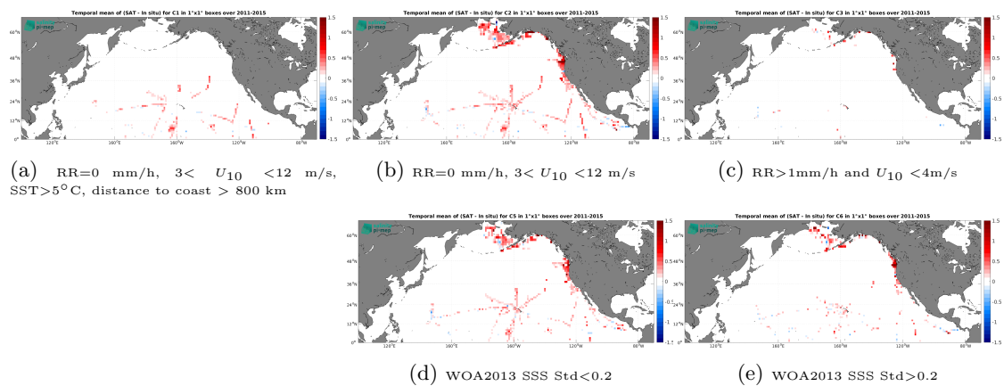
Figure 14: Temporal mean gridded over spatial boxes of size 1^\circ \times 1^\circ of \Delta\text{SSS} (Aquarius SSS L3 CAP v5 - Monthly (JPL) - TSG (SAMOS)) for 5 different subdatasets corresponding to: RR=0 mm/h, 3 < U_{10} < 12 m/s, SST > 5°C, distance to coast > 800 km (a), RR=0 mm/h, 3 < U_{10} < 12 m/s (b), RR > 1mm/h and U_{10} < 4 m/s (c), WOA2013 SSS Std < 0.2 (d), WOA2013 SSS Std > 0.2 (e).
