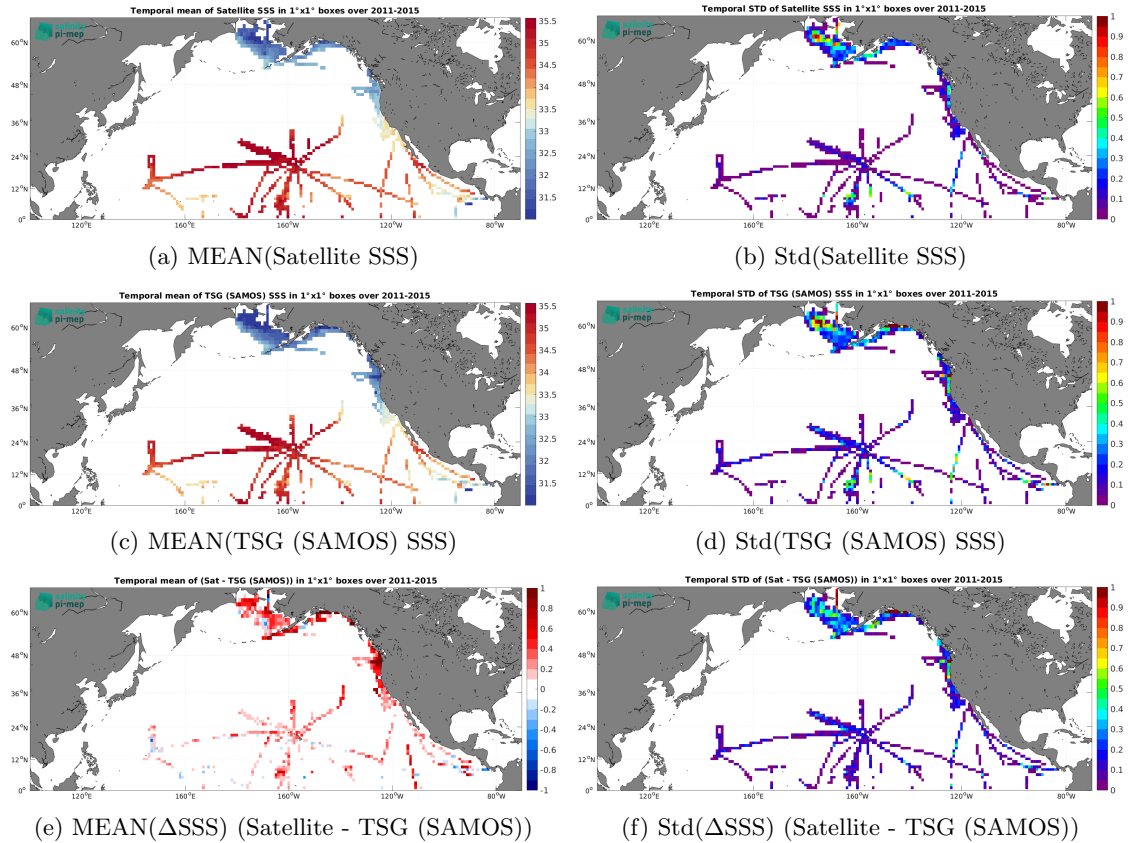
Figure 7: Temporal mean (left) and Std (right) of SSS from Aquarius SSS L3 CAP v5 - Monthly (JPL) (top), TSG (SAMOS) (middle), and of \Delta SSS (Satellite - TSG (SAMOS)). Only match-up pairs are used to generate these maps.
