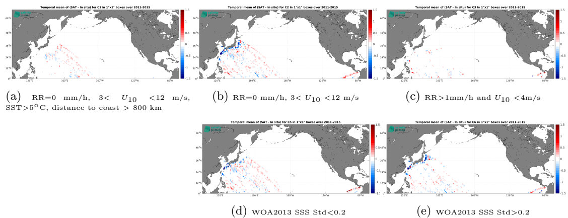
Figure 14: Temporal mean gridded over spatial boxes of size 1^\circ \times 1^\circ of \Delta SSS (Aquarius SSS L3 CAP v5 - Monthly (JPL) - TSG (LEGOS-DM)) for 5 different subdatasets corresponding to:RR=0 mm/h, 3 < U_{10} < 12 m/s, SST >5^\circ\text{C} , distance to coast > 800 km (a), RR=0 mm/h, 3 < U_{10} < 12 m/s (b), RR >1 mm/h and U_{10} < 4 m/s (c), WOA2013 SSS Std <0.2 (d), WOA2013 SSS Std >0.2 (e).
