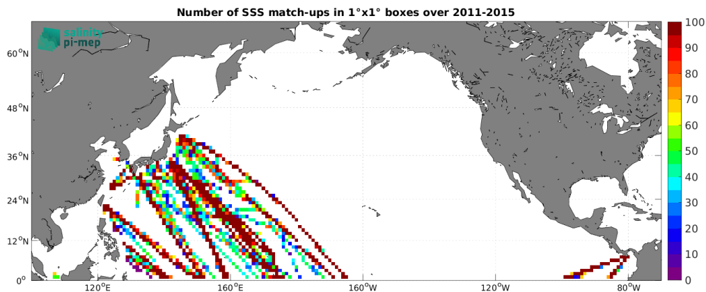
Figure 5: Number of SSS match-ups between TSG (LEGOS-DM) SSS and the Aquarius SSS L3 CAP v5 - Monthly (JPL) SSS product for the North Pacific Ocean Pi-MEP region over 1^\circ \times 1^\circ boxes and for the full satellite product period.
