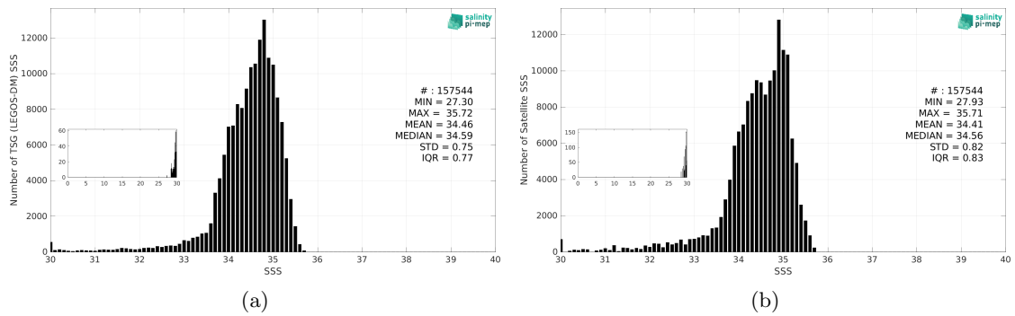
Figure 3: Histograms of SSS from TSG (LEGOS-DM) (a) and Aquarius SSS L3 CAP v5 - Monthly (JPL) (b) considering all match-up pairs per bins of 0.1 over the North Pacific Ocean Pi-MEP region and for the full satellite product period.
