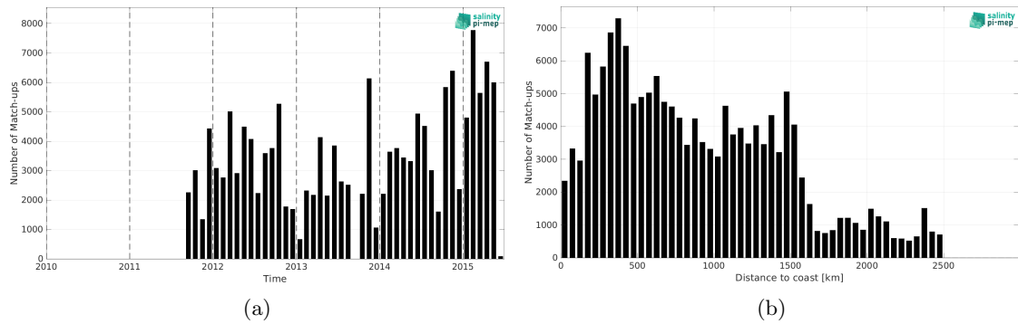
Figure 2: Number of match-ups between TSG (LEGOS-DM) and Aquarius SSS L3 CAP v5 - Monthly (JPL) SSS as a function of time (a) and as function of the distance to coast (b) over the North Pacific Ocean Pi-MEP region and for the full satellite product period.
