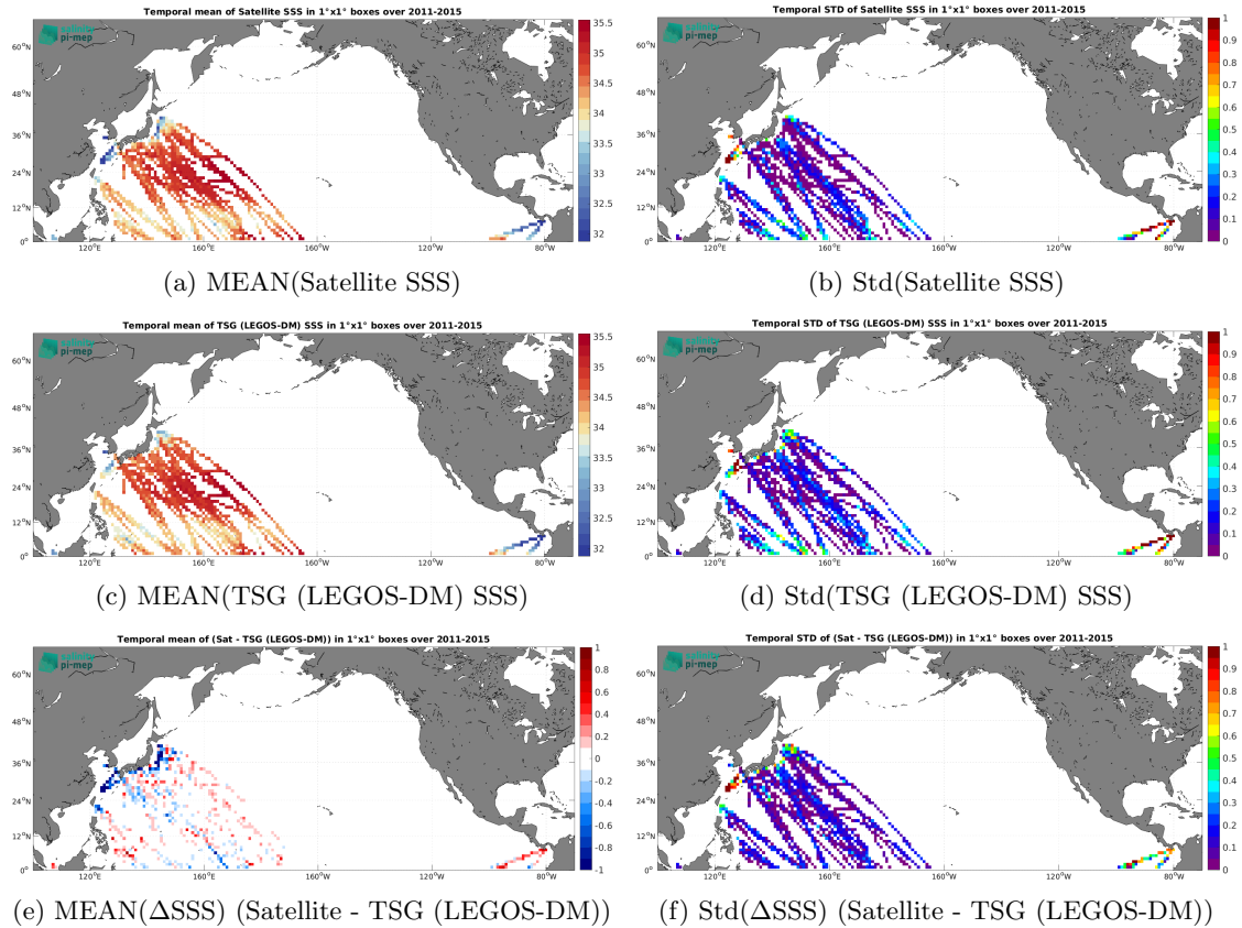
Figure 7: Temporal mean (left) and Std (right) of SSS from Aquarius SSS L3 CAP v5 - Monthly (JPL) (top), TSG (LEGOS-DM) (middle), and of \Delta SSS (Satellite - TSG (LEGOS-DM)). Only match-up pairs are used to generate these maps.
