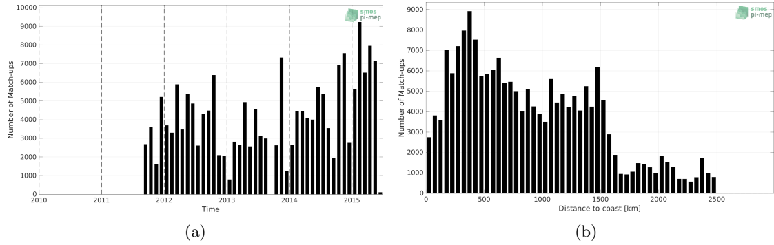
Figure 1: Number of match-ups between TSG (LEGOS-DM) and Aquarius SSS L3 CAP v5 - Monthly (JPL) SSS as a function of time (a) and as function of the distance to coast (b) over the North Pacific Ocean Pi-MEP region and for the full satellite product period.
