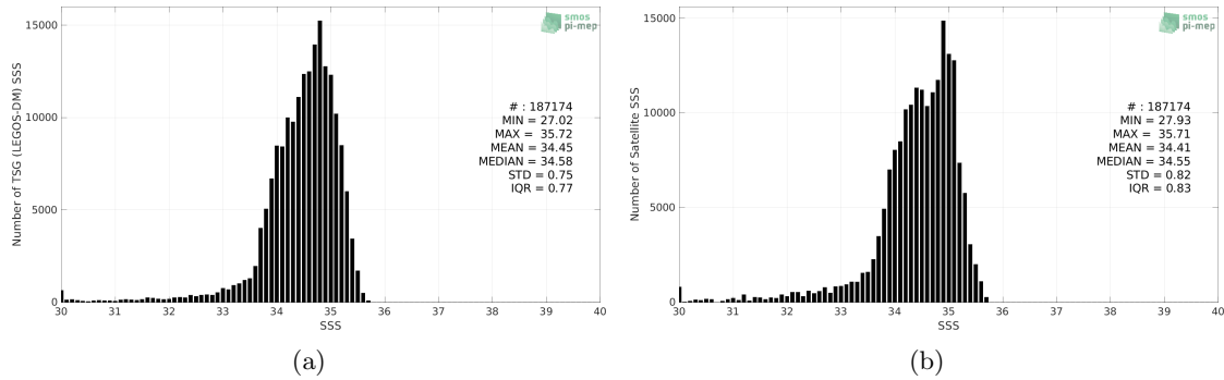
Figure 2: Histograms of SSS from TSG (LEGOS-DM) (a) and Aquarius SSS L3 CAP v5 - Monthly (JPL) (b) considering all match-up pairs per bins of 0.1 over the North Pacific Ocean Pi-MEP region and for the full satellite product period.
