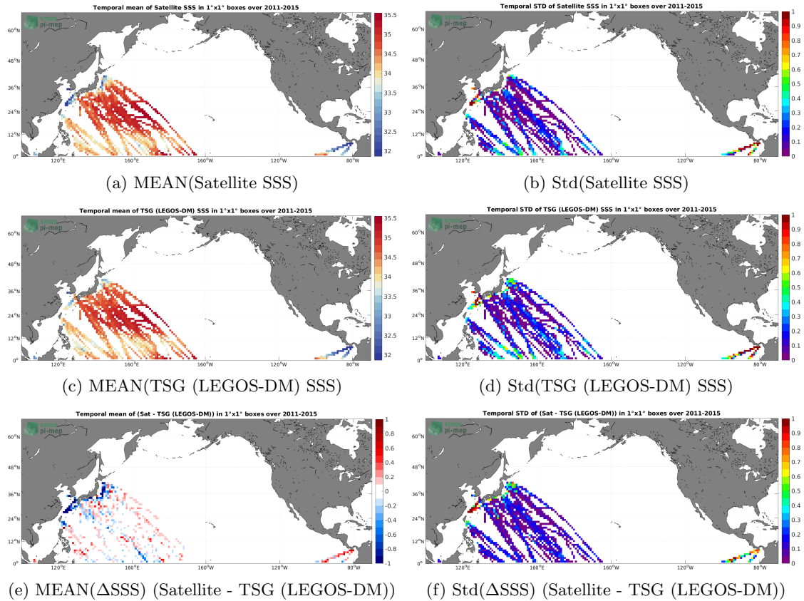
Figure 6: Temporal mean (left) and Std (right) of SSS from Aquarius SSS L3 CAP v5 - Monthly (JPL) (top), TSG (LEGOS-DM) (middle), and of \Delta SSS (Satellite - TSG (LEGOS-DM)). Only match-up pairs are used to generate these maps.
