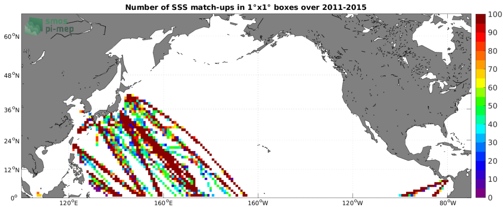
Figure 4: Number of SSS match-ups between TSG (LEGOS-DM) SSS and the Aquarius SSS L3 CAP v5 - Monthly (JPL) SSS product for the North Pacific Ocean Pi-MEP region over 1^\circ \times 1^\circ boxes and for the full satellite product period.
