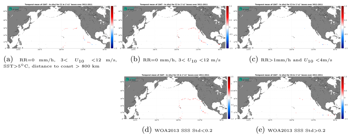
Figure 12: Temporal mean gridded over spatial boxes of size 1^\circ \times 1^\circ of \Delta\text{SSS} (Aquarius SSS L3 CAP v5 - Monthly (JPL) - TSG (GOSUD-Sailing-ship)) for 5 different subdatasets corresponding to:RR=0 mm/h, 3 < U_{10} < 12 m/s, SST>5°C, distance to coast > 800 km (a), RR=0 mm/h, 3 < U_{10} < 12 m/s (b), RR>1mm/h and U_{10} < 4 m/s (c), WOA2013 SSS Std<0.2 (d), WOA2013 SSS Std>0.2 (e).
