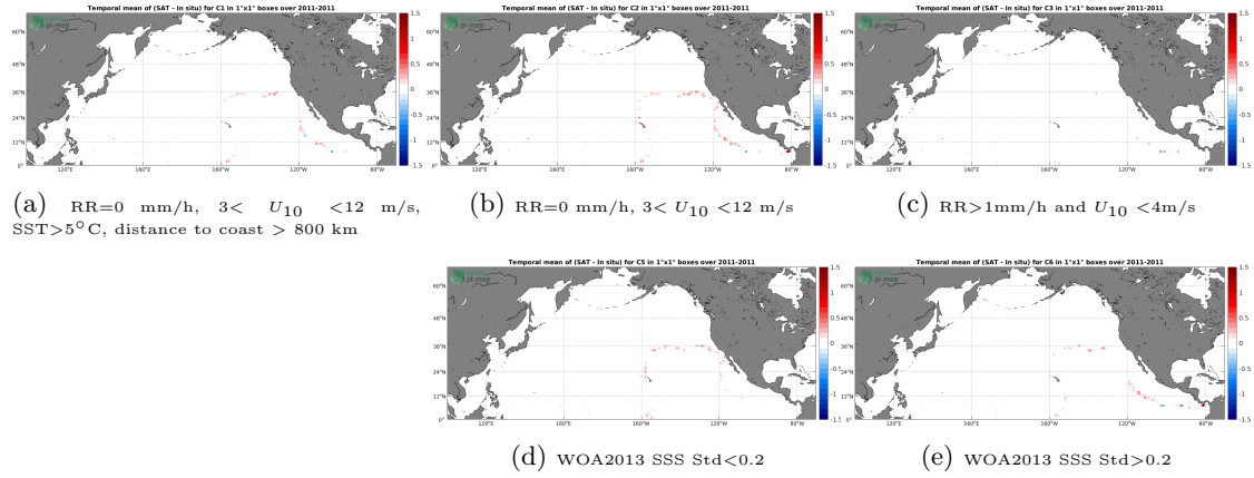
Figure 12: Temporal mean gridded over spatial boxes of size 1^\circ \times 1^\circ of \Delta SSS (Aquarius SSS L3 CAP v5 - Monthly (JPL) - TSG (GOSUD-Sailing-ship)) for 5 different subdatasets corresponding to: RR=0 mm/h, 3 < U_{10} < 12 m/s, SST>5°C, distance to coast > 800 km (a), RR=0 mm/h, 3 < U_{10} < 12 m/s (b), RR>1mm/h and U_{10} < 4 m/s (c), WOA2013 SSS Std<0.2 (d), WOA2013 SSS Std>0.2 (e).
