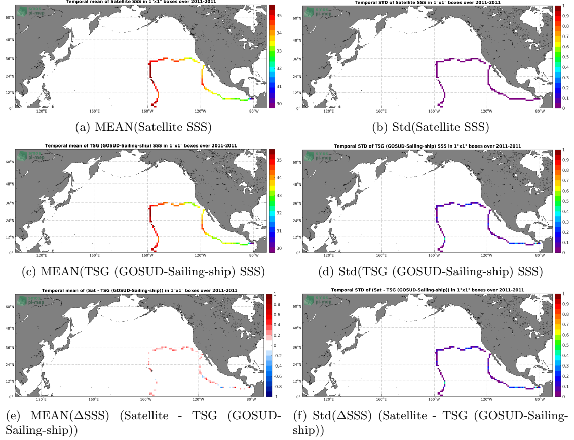
Figure 6: Temporal mean (left) and Std (right) of SSS from Aquarius SSS L3 CAP v5 - Monthly (JPL) (top), TSG (GOSUD-Sailing-ship) (middle), and of \Delta\text{SSS} (Satellite - TSG (GOSUD-Sailing-ship)). Only match-up pairs are used to generate these maps.
