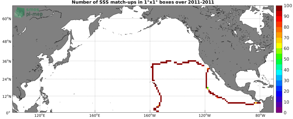
Figure 4: Number of SSS match-ups between TSG (GOSUD-Sailing-ship) SSS and the Aquarius SSS L3 CAP v5 - Monthly (JPL) SSS product for the North Pacific Ocean Pi-MEP region over 1^\circ \times 1^\circ boxes and for the full satellite product period.
