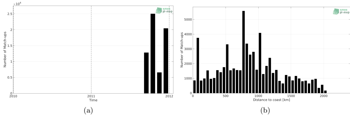
Figure 1: Number of match-ups between TSG (GOSUD-Sailing-ship) and Aquarius SSS L3 CAP v5 - Monthly (JPL) SSS as a function of time (a) and as function of the distance to coast (b) over the North Pacific Ocean Pi-MEP region and for the full satellite product period.
