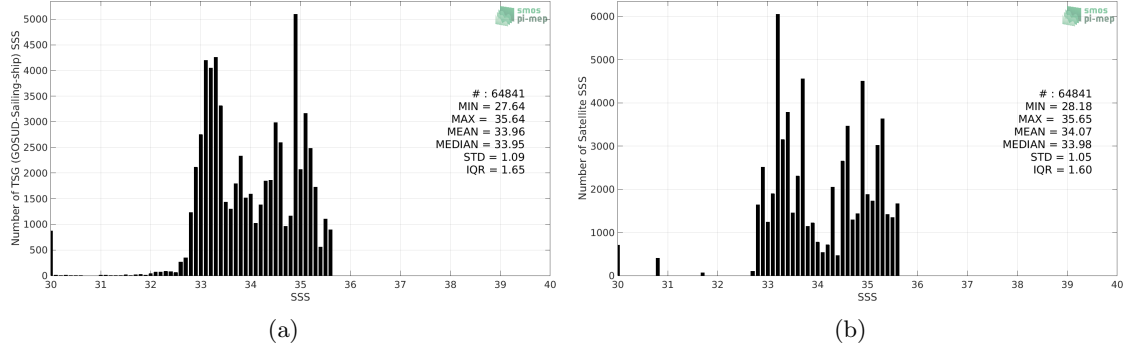
Figure 2: Histograms of SSS from TSG (GOSUD-Sailing-ship) (a) and Aquarius SSS L3 CAP v5 - Monthly (JPL) (b) considering all match-up pairs per bins of 0.1 over the North Pacific Ocean Pi-MEP region and for the full satellite product period.
