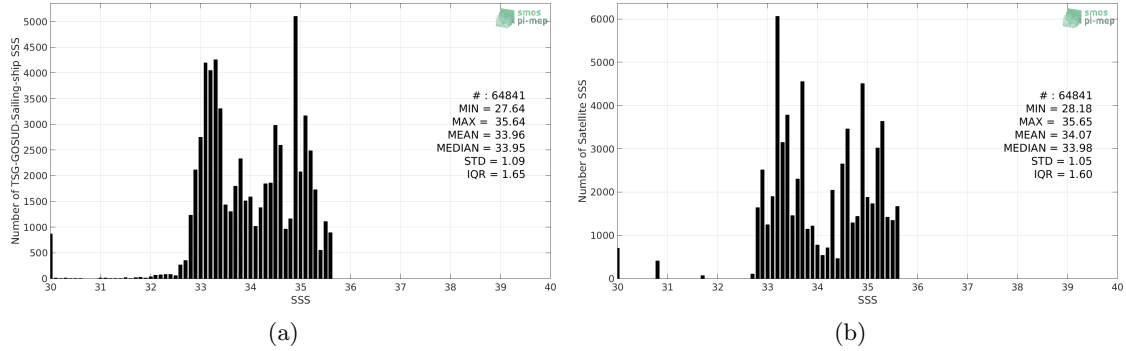
Figure 2: Histograms of SSS from TSG-GOSUD-Sailing-ship (a) and Aquarius-L3-JPL-V5-MONTHLY (b) considering all match-up pairs per bins of 0.1 over the North Pacific Ocean Pi-MEP region and for the full satellite product period.
