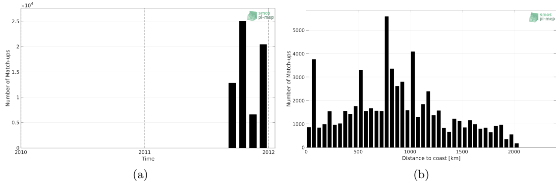
Figure 1: Number of match-ups between TSG-GOSUD-Sailing-ship and Aquarius-L3-JPL-V5-MONTHLY SSS as a function of time (a) and as function of the distance to coast (b) over the North Pacific Ocean Pi-MEP region and for the full satellite product period.
