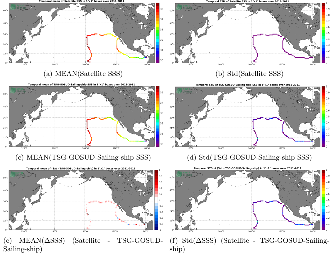
Figure 6: Temporal mean (left) and Std (right) of SSS from Aquarius-L3-JPL-V5-MONTHLY (top), TSG-GOSUD-Sailing-ship (middle), and of \Delta\text{SSS} (Satellite - TSG-GOSUD-Sailing-ship). Only match-up pairs are used to generate these maps.
