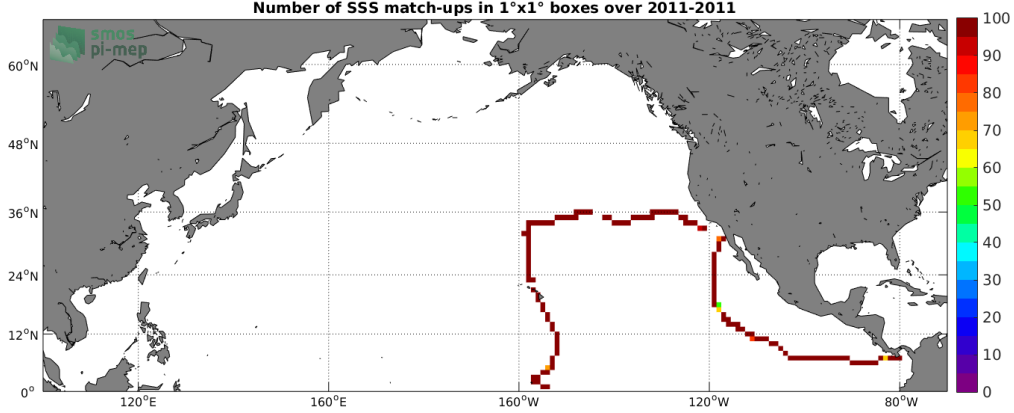
Figure 4: Number of SSS match-ups between TSG-GOSUD-Sailing-ship SSS and the Aquarius-L3-JPL-V5-MONTHLY SSS product for the North Pacific Ocean Pi-MEP region over 1^\circ \times 1^\circ boxes and for the full satellite product period.
