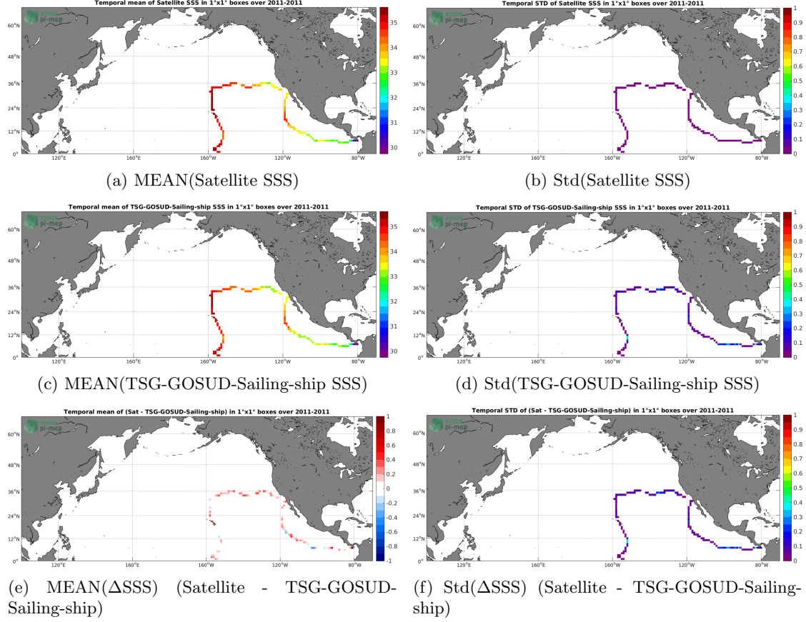
Figure 6: Temporal mean (left) and Std (right) of SSS from Aquarius-L3-JPL-V5-MONTHLY (top), TSG-GOSUD-Sailing-ship (middle), and of \Delta SSS (Satellite - TSG-GOSUD-Sailing-ship). Only match-up pairs are used to generate these maps.
