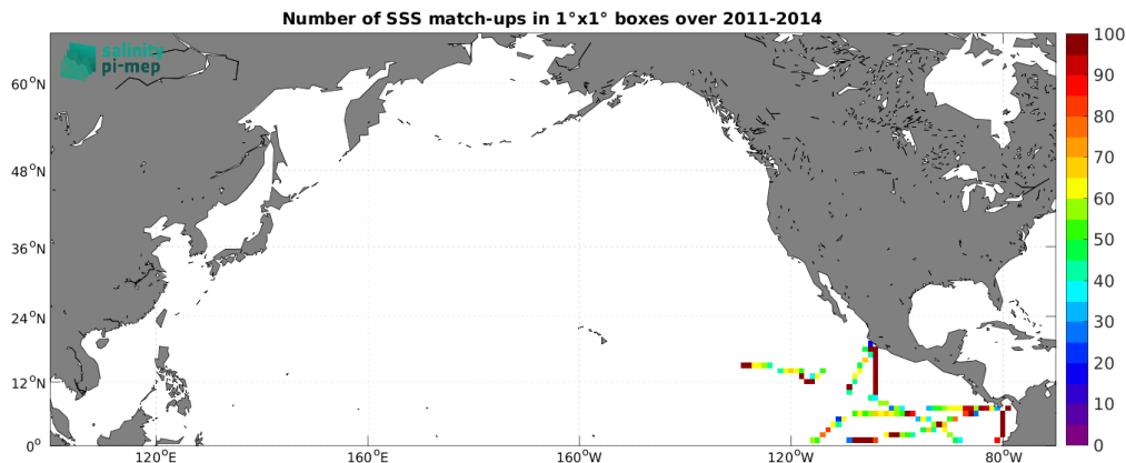
Figure 5: Number of SSS match-ups between TSG (GOSUD-Research-vessel) SSS and the Aquarius SSS L3 CAP v5 - Monthly (JPL) SSS product for the North Pacific Ocean Pi-MEP region over 1^\circ \times 1^\circ boxes and for the full satellite product period.
