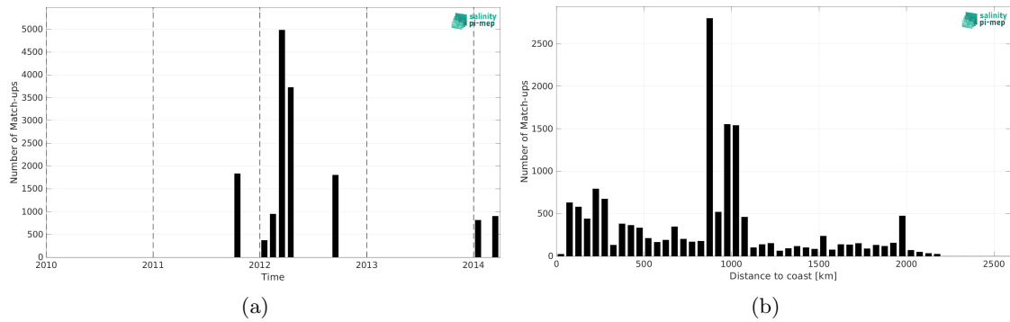
Figure 2: Number of match-ups between TSG (GOSUD-Research-vessel) and Aquarius SSS L3 CAP v5 - Monthly (JPL) SSS as a function of time (a) and as function of the distance to coast (b) over the North Pacific Ocean Pi-MEP region and for the full satellite product period.
