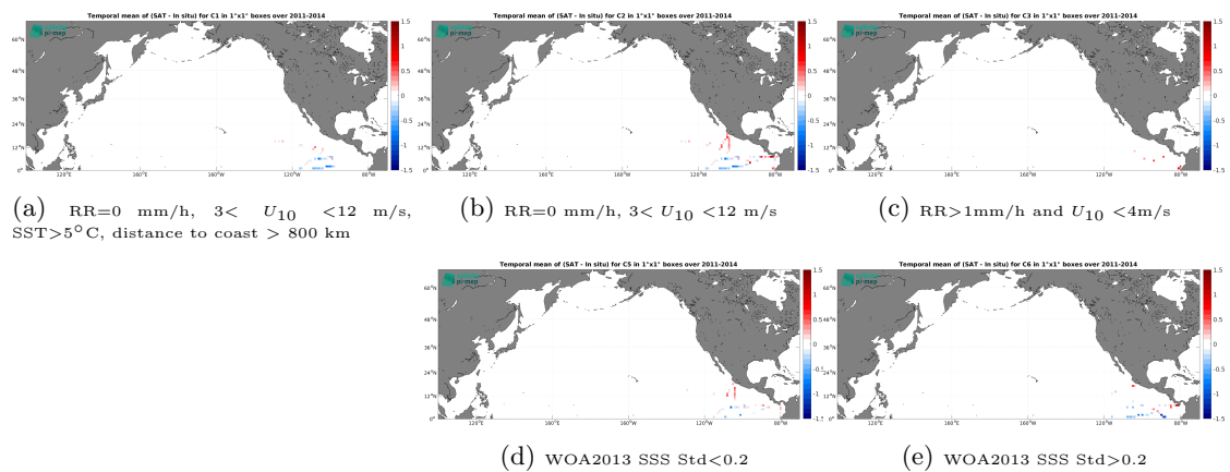
Figure 14: Temporal mean gridded over spatial boxes of size 1^\circ \times 1^\circ of \Delta\text{SSS} (Aquarius SSS L3 CAP v5 - Monthly (JPL) - TSG (GOSUD-Research-vessel)) for 5 different subdatasets corresponding to:RR=0 mm/h, 3 < U_{10} < 12 m/s, SST >5^\circ\text{C} , distance to coast > 800 km (a), RR=0 mm/h, 3 < U_{10} < 12 m/s (b), RR >1 mm/h and U_{10} < 4 m/s (c), WOA2013 SSS Std <0.2 (d), WOA2013 SSS Std >0.2 (e).
