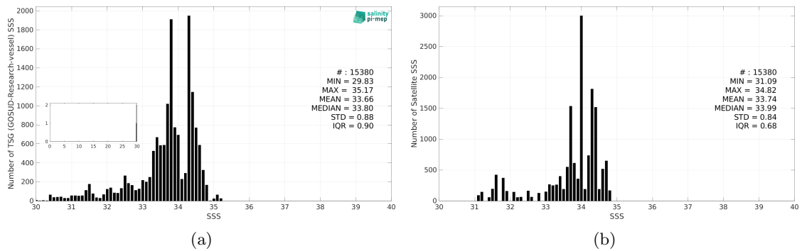
Figure 3: Histograms of SSS from TSG (GOSUD-Research-vessel) (a) and Aquarius SSS L3 CAP v5 - Monthly (JPL) (b) considering all match-up pairs per bins of 0.1 over the North Pacific Ocean Pi-MEP region and for the full satellite product period.
