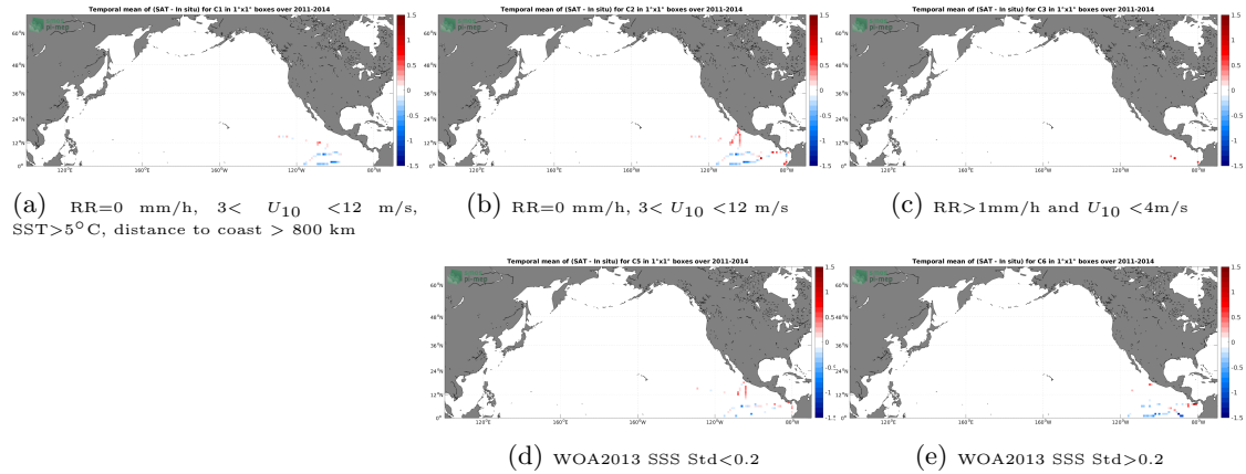
Figure 12: Temporal mean gridded over spatial boxes of size 1^{\circ}\times 1^{\circ} of \Delta SSS (Aquarius SSS L3 CAP v5 - Monthly (JPL) - TSG (GOSUD-Research-vessel)) for 5 different subdatasets corresponding to:RR=0 mm/h, 3 < U_{10} < 12 m/s, SST > 5^{\circ}\text{C} , distance to coast > 800 km (a), RR=0 mm/h, 3 < U_{10} < 12 m/s (b), RR > 1 mm/h and U_{10} < 4 m/s (c), WOA2013 SSS Std < 0.2 (d), WOA2013 SSS Std > 0.2 (e).
