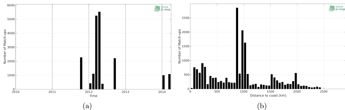
Figure 1: Number of match-ups between TSG-GOSUD-Research-vessel and Aquarius-L3-JPL-V5-MONTHLY SSS as a function of time (a) and as function of the distance to coast (b) over the North Pacific Ocean Pi-MEP region and for the full satellite product period.
