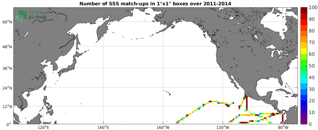
Figure 4: Number of SSS match-ups between TSG-GOSUD-Research-vessel SSS and the Aquarius-L3-JPL-V5-MONTHLY SSS product for the North Pacific Ocean Pi-MEP region over 1°x1° boxes and for the full satellite product period.
