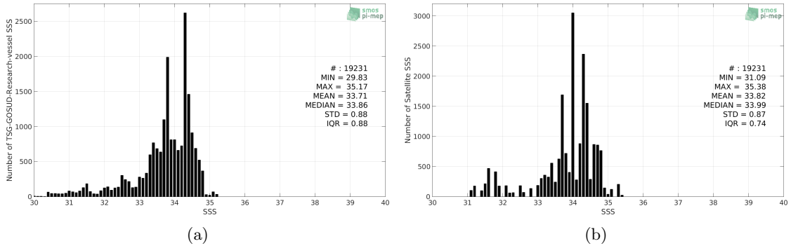
Figure 2: Histograms of SSS from TSG-GOSUD-Research-vessel (a) and Aquarius-L3-JPL-V5-MONTHLY (b) considering all match-up pairs per bins of 0.1 over the North Pacific Ocean Pi-MEP region and for the full satellite product period.
