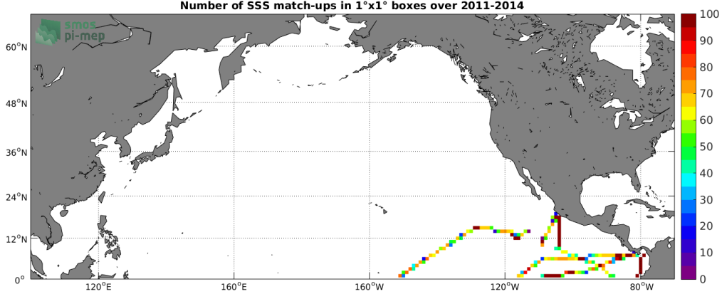
Figure 4: Number of SSS match-ups between TSG-GOSUD-Research-vessel SSS and the Aquarius-L3-JPL-V5-MONTHLY SSS product for the North Pacific Ocean Pi-MEP region over 1^\circ \times 1^\circ boxes and for the full satellite product period.
