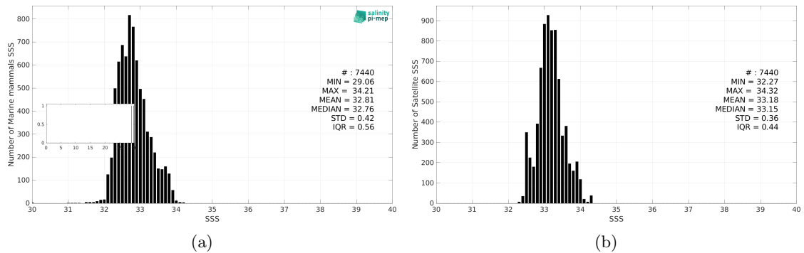
Figure 3: Histograms of SSS from Marine mammals (a) and Aquarius SSS L3 CAP v5 - Monthly (JPL) (b) considering all match-up pairs per bins of 0.1 over the North Pacific Ocean Pi-MEP region and for the full satellite product period.
