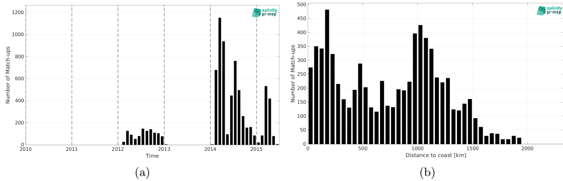
Figure 2: Number of match-ups between Marine mammals and Aquarius SSS L3 CAP v5 - Monthly (JPL) SSS as a function of time (a) and as function of the distance to coast (b) over the North Pacific Ocean Pi-MEP region and for the full satellite product period.
