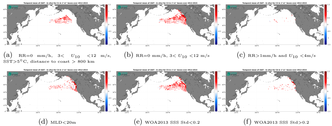
Figure 14: Temporal mean gridded over spatial boxes of size 1^\circ \times 1^\circ of \Delta SSS (Aquarius SSS L3 CAP v5 - Monthly (JPL) - Marine mammals) for 6 different subdatasets corresponding to:RR=0 mm/h, 3 < U_{10} < 12 m/s, SST>5°C, distance to coast > 800 km (a), RR=0 mm/h, 3 < U_{10} < 12 m/s (b), RR>1mm/h and U_{10} < 4 m/s (c),MLD<20m (d),WOA2013 SSS Std<0.2 (e),WOA2013 SSS Std>0.2 (f).
