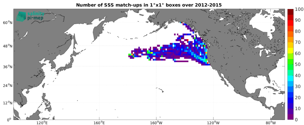
Figure 5: Number of SSS match-ups between Marine mammals SSS and the Aquarius SSS L3 CAP v5 - Monthly (JPL) SSS product for the North Pacific Ocean Pi-MEP region over 1^\circ \times 1^\circ boxes and for the full satellite product period.
