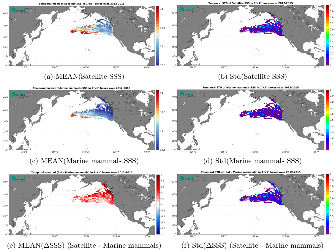
Figure 7: Temporal mean (left) and Std (right) of SSS from Aquarius SSS L3 CAP v5 - Monthly (JPL) (top), Marine mammals (middle), and of \Delta SSS (Satellite - Marine mammals). Only match-up pairs are used to generate these maps.
